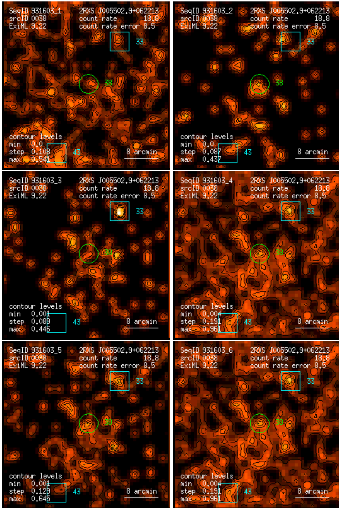
Figure 38: RASS 931603: detection 0038: band rate images, Gaussian filter: (1) PSPC channels 11 – 41, (2) 52 – 90, (3) 91 – 201, (4) 11 – 235, (5) 52 – 201, (6) 11 – 201. Broad band rates in counts/ks. Band rate contour levels in counts/ks/arcmin 2 .
