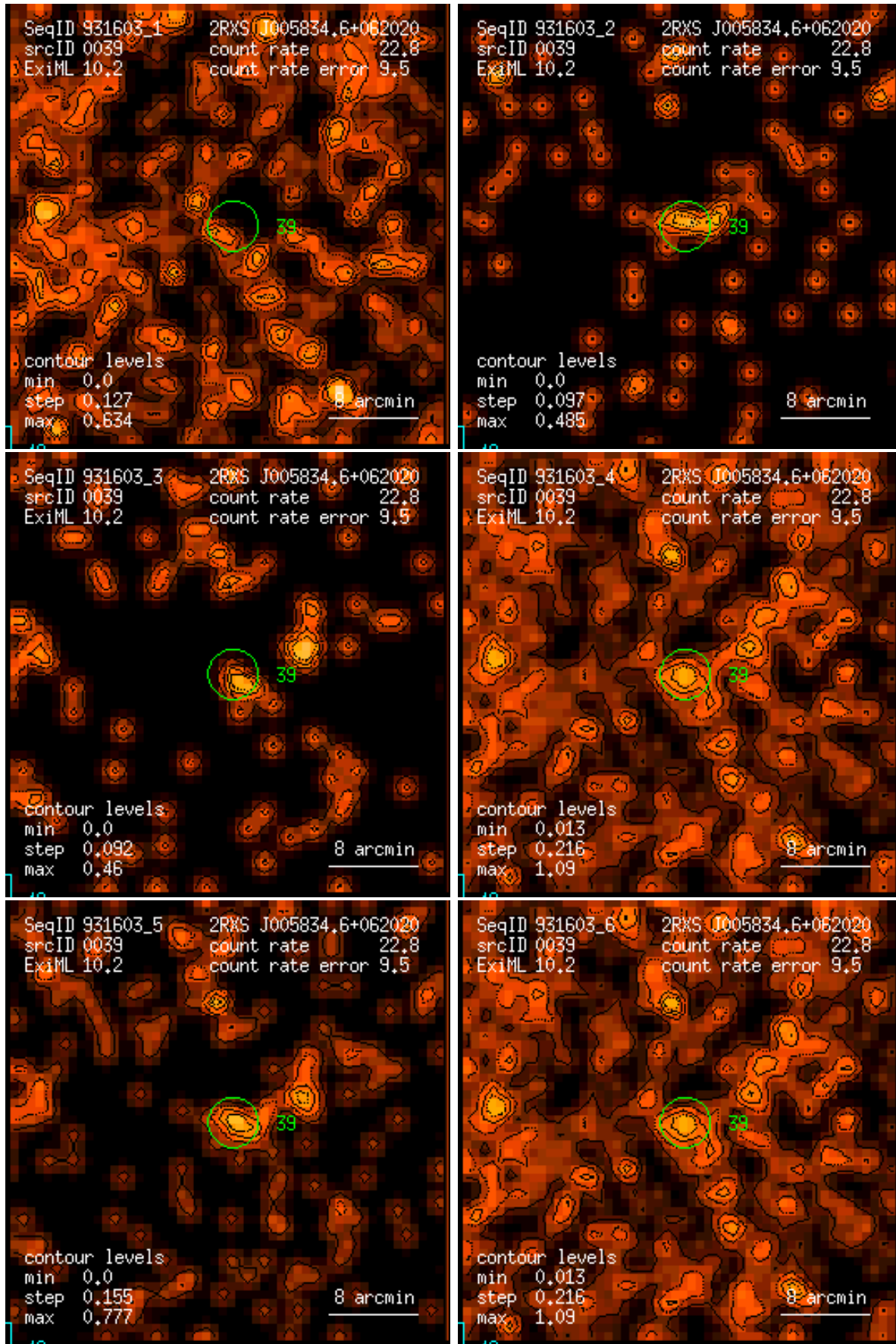
Figure 39: RASS 931603: detection 0039: band rate images, Gaussian filter: (1) PSPC channels 11 – 41, (2) 52 – 90, (3) 91 – 201, (4) 11 – 235, (5) 52 – 201, (6) 11 – 201. Broad band rates in counts/ks. Band rate contour levels in counts/ks/arcmin 2 .
