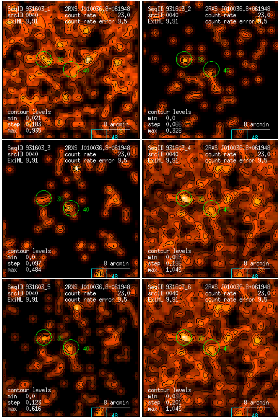
Figure 40: RASS 931603: detection 0040: band rate images, Gaussian filter: (1) PSPC channels 11 – 41, (2) 52 – 90, (3) 91 – 201, (4) 11 – 235, (5) 52 – 201, (6) 11 – 201. Broad band rates in counts/ks. Band rate contour levels in counts/ks/arcmin 2 .
