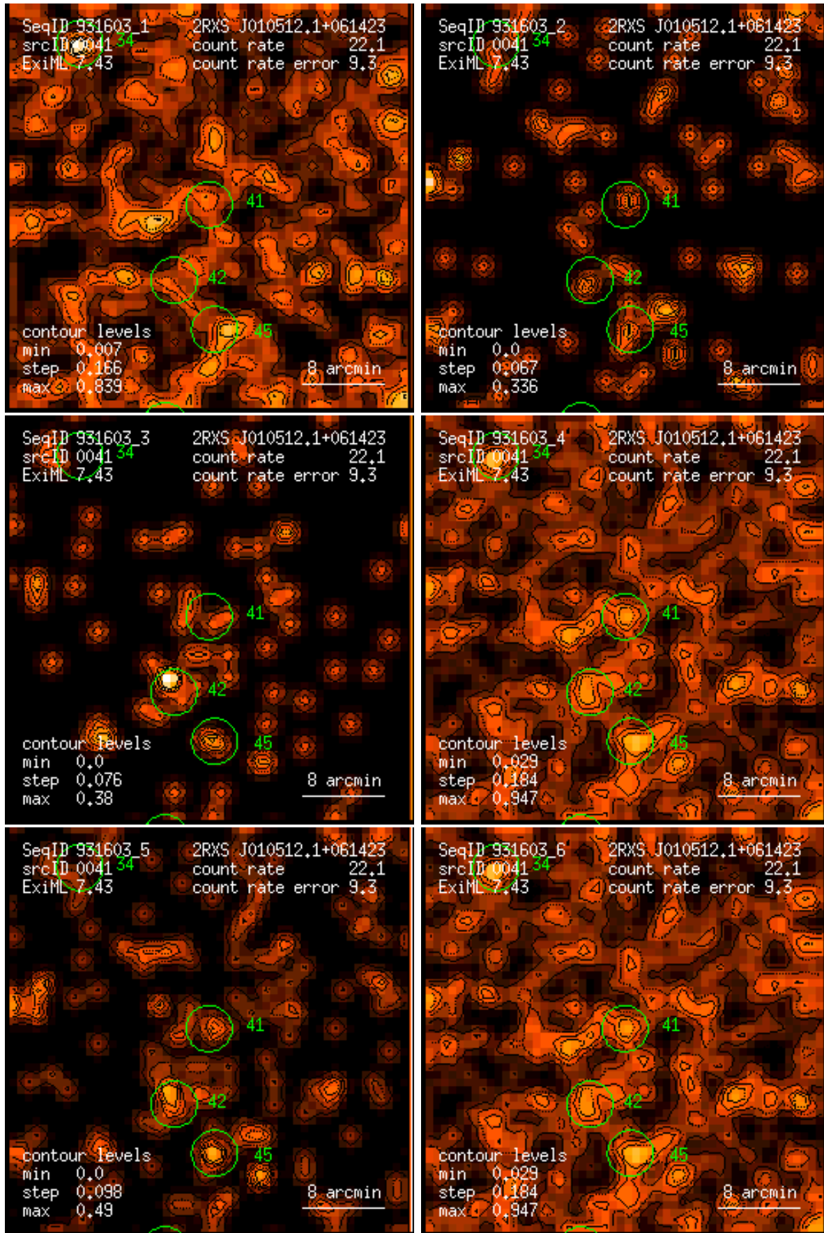
Figure 41: RASS 931603: detection 0041: band rate images, Gaussian filter: (1) PSPC channels 11 – 41, (2) 52 – 90, (3) 91 – 201, (4) 11 – 235, (5) 52 – 201, (6) 11 – 201. Broad band rates in counts/ks. Band rate contour levels in counts/ks/arcmin 2 .
