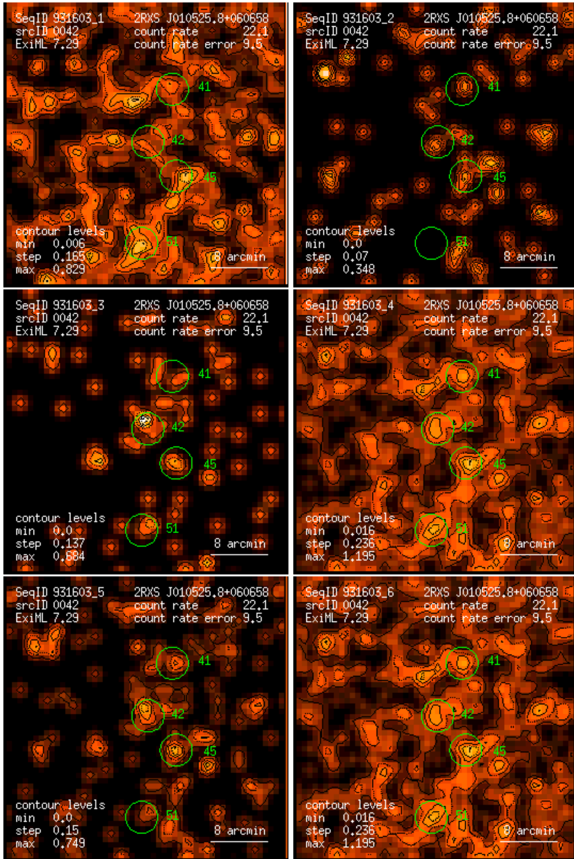
Figure 42: RASS 931603: detection 0042: band rate images, Gaussian filter: (1) PSPC channels 11 – 41, (2) 52 – 90, (3) 91 – 201, (4) 11 – 235, (5) 52 – 201, (6) 11 – 201. Broad band rates in counts/ks. Band rate contour levels in counts/ks/arcmin 2 .
