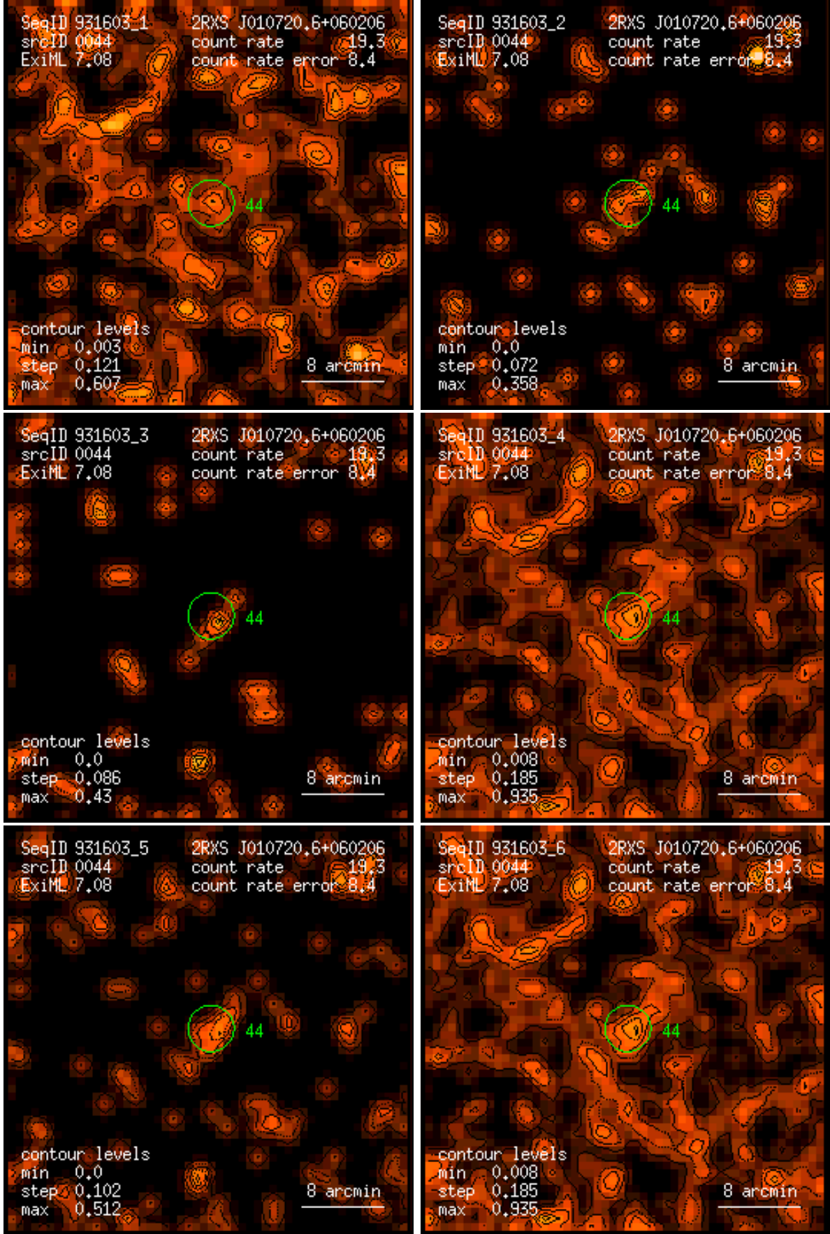
Figure 44: RASS 931603: detection 0044: band rate images, Gaussian filter: (1) PSPC channels 11 – 41, (2) 52 – 90, (3) 91 – 201, (4) 11 – 235, (5) 52 – 201, (6) 11 – 201. Broad band rates in counts/ks. Band rate contour levels in counts/ks/arcmin 2 .
