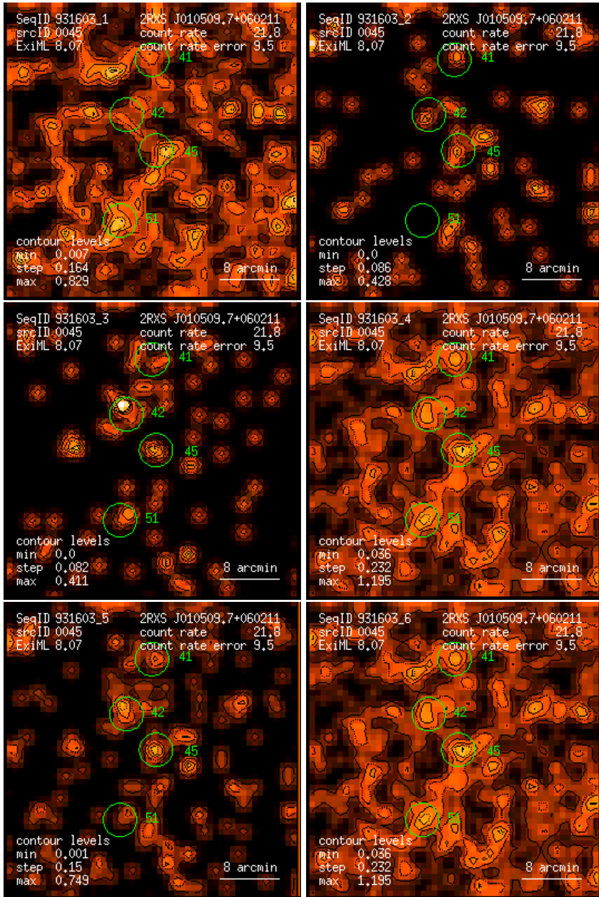
Figure 45: RASS 931603: detection 0045: band rate images, Gaussian filter: (1) PSPC channels 11 – 41, (2) 52 – 90, (3) 91 – 201, (4) 11 – 235, (5) 52 – 201, (6) 11 – 201. Broad band rates in counts/ks. Band rate contour levels in counts/ks/arcmin 2 .
