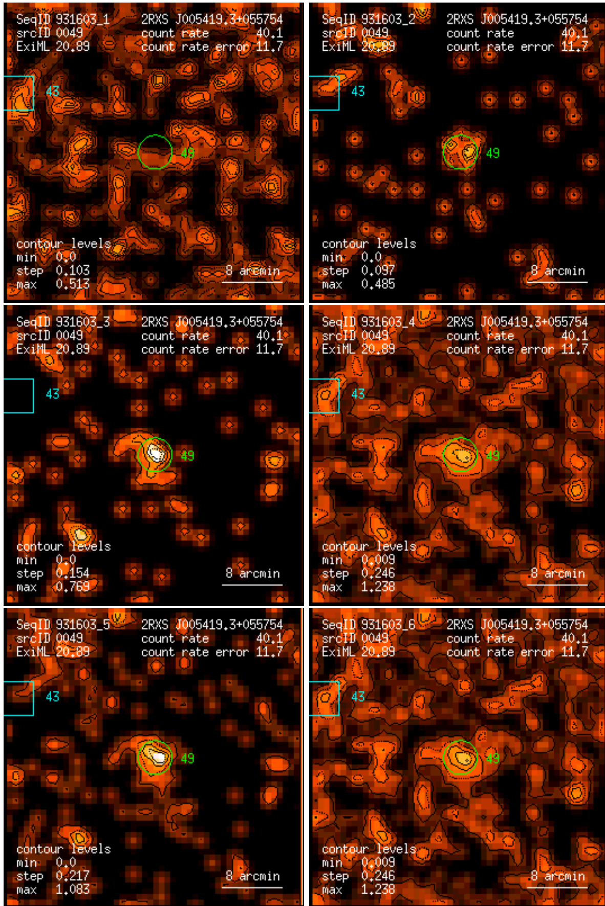
Figure 49: RASS 931603: detection 0049: band rate images, Gaussian filter: (1) PSPC channels 11 – 41, (2) 52 – 90, (3) 91 – 201, (4) 11 – 235, (5) 52 – 201, (6) 11 – 201. Broad band rates in counts/ks. Band rate contour levels in counts/ks/arcmin 2 .
