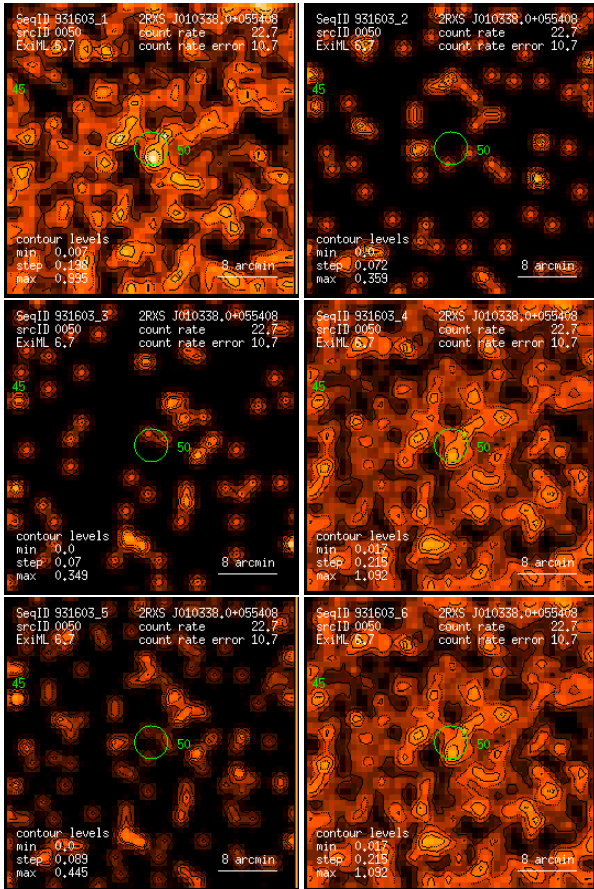
Figure 50: RASS 931603: detection 0050: band rate images, Gaussian filter: (1) PSPC channels 11 – 41, (2) 52 – 90, (3) 91 – 201, (4) 11 – 235, (5) 52 – 201, (6) 11 – 201. Broad band rates in counts/ks. Band rate contour levels in counts/ks/arcmin 2 .
