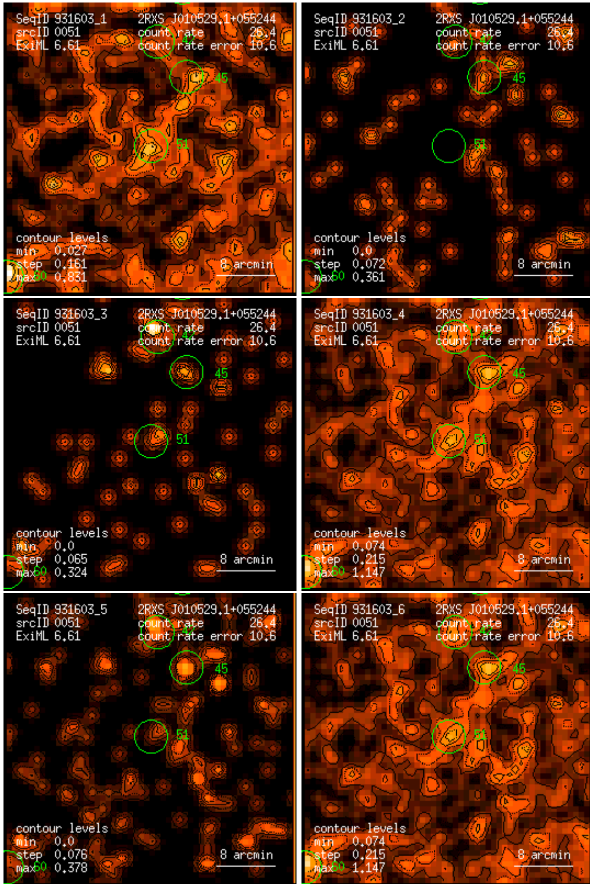
Figure 51: RASS 931603: detection 0051: band rate images, Gaussian filter: (1) PSPC channels 11 – 41, (2) 52 – 90, (3) 91 – 201, (4) 11 – 235, (5) 52 – 201, (6) 11 – 201. Broad band rates in counts/ks. Band rate contour levels in counts/ks/arcmin 2 .
