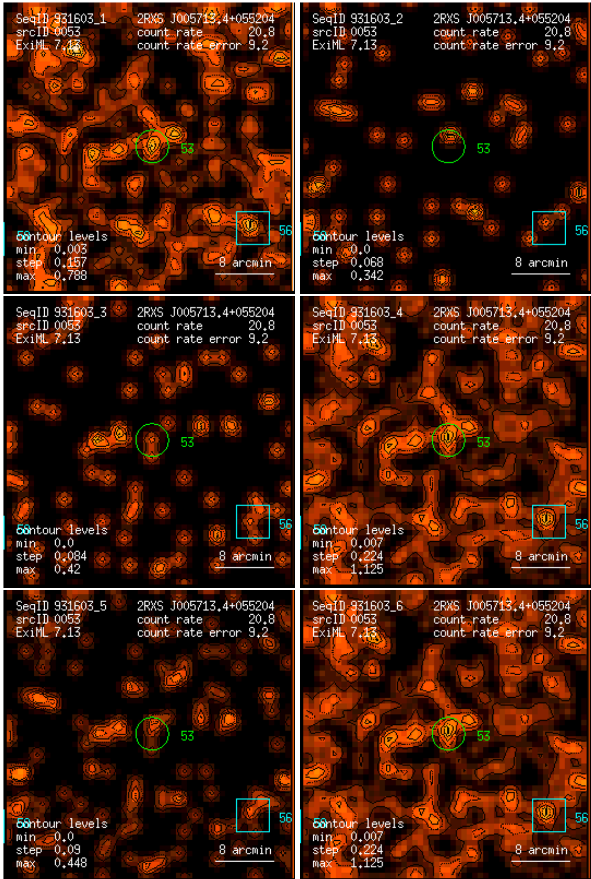
Figure 53: RASS 931603: detection 0053: band rate images, Gaussian filter: (1) PSPC channels 11 – 41, (2) 52 – 90, (3) 91 – 201, (4) 11 – 235, (5) 52 – 201, (6) 11 – 201. Broad band rates in counts/ks. Band rate contour levels in counts/ks/arcmin 2 .
