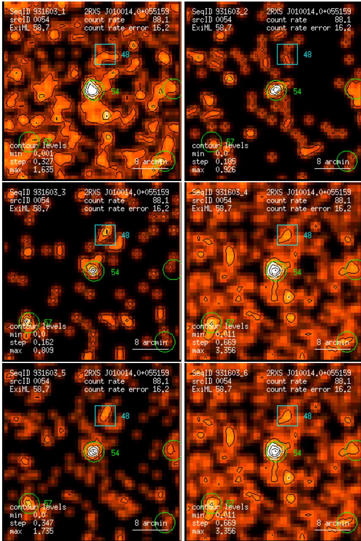
Figure 54: RASS 931603: detection 0054: band rate images, Gaussian filter: (1) PSPC channels 11 – 41, (2) 52 – 90, (3) 91 – 201, (4) 11 – 235, (5) 52 – 201, (6) 11 – 201. Broad band rates in counts/ks. Band rate contour levels in counts/ks/arcmin 2 .
