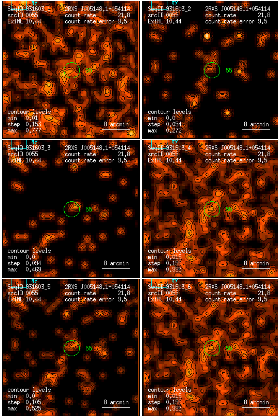
Figure 55: RASS 931603: detection 0055: band rate images, Gaussian filter: (1) PSPC channels 11 – 41, (2) 52 – 90, (3) 91 – 201, (4) 11 – 235, (5) 52 – 201, (6) 11 – 201. Broad band rates in counts/ks. Band rate contour levels in counts/ks/arcmin 2 .
