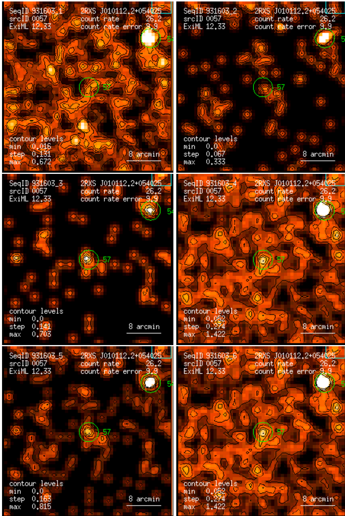
Figure 57: RASS 931603: detection 0057: band rate images, Gaussian filter: (1) PSPC channels 11 – 41, (2) 52 – 90, (3) 91 – 201, (4) 11 – 235, (5) 52 – 201, (6) 11 – 201. Broad band rates in counts/ks. Band rate contour levels in counts/ks/arcmin 2 .
