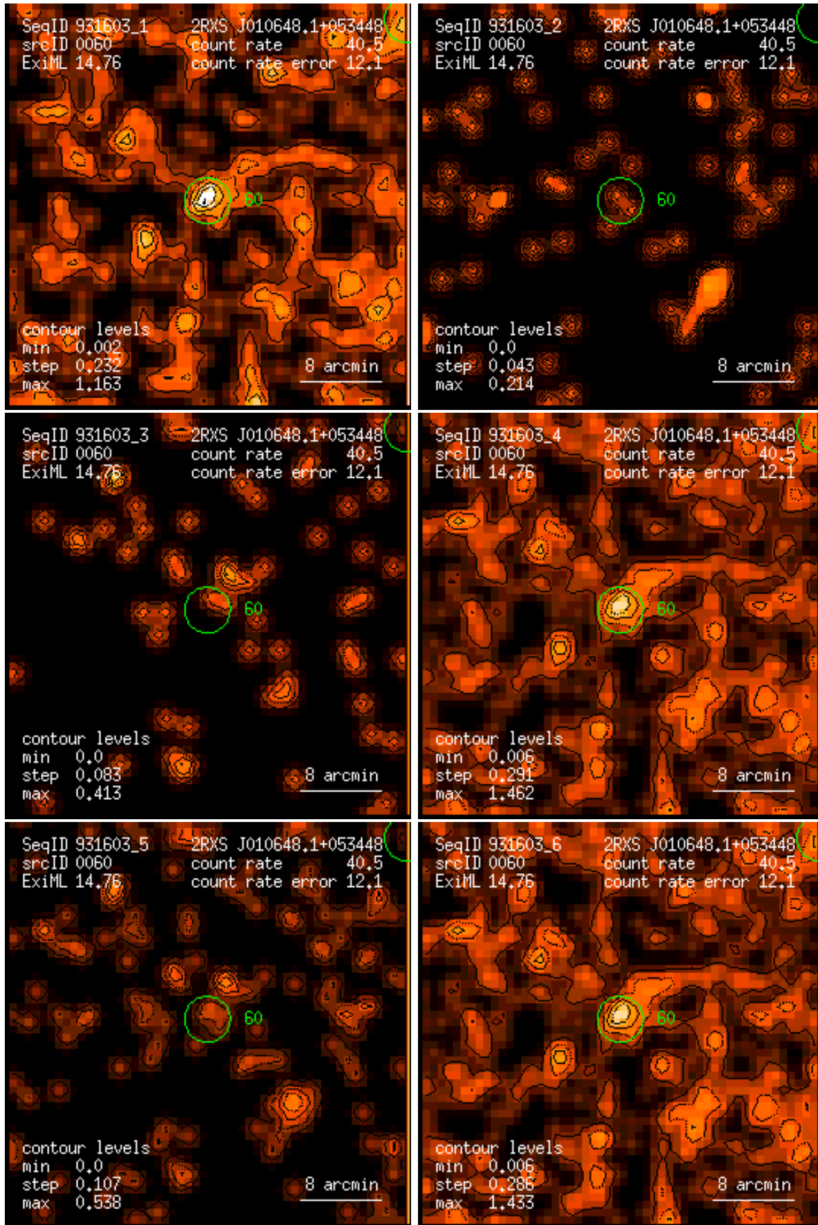
Figure 60: RASS 931603: detection 0060: band rate images, Gaussian filter: (1) PSPC channels 11 – 41, (2) 52 – 90, (3) 91 – 201, (4) 11 – 235, (5) 52 – 201, (6) 11 – 201. Broad band rates in counts/ks. Band rate contour levels in counts/ks/arcmin 2 .
