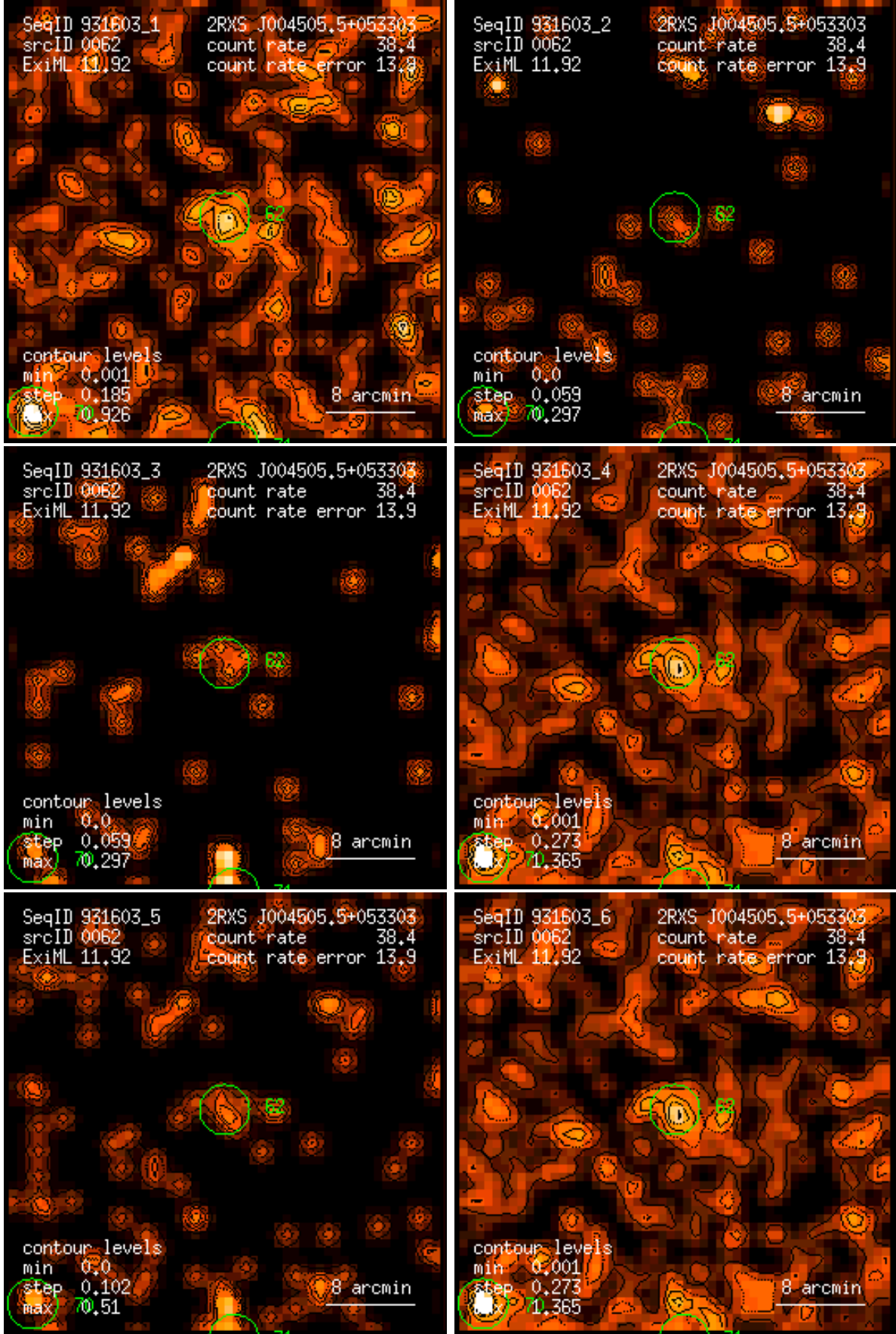
Figure 62: RASS 931603: detection 0062: band rate images, Gaussian filter: (1) PSPC channels 11 – 41, (2) 52 – 90, (3) 91 – 201, (4) 11 – 235, (5) 52 – 201, (6) 11 – 201. Broad band rates in counts/ks. Band rate contour levels in counts/ks/arcmin 2 .
