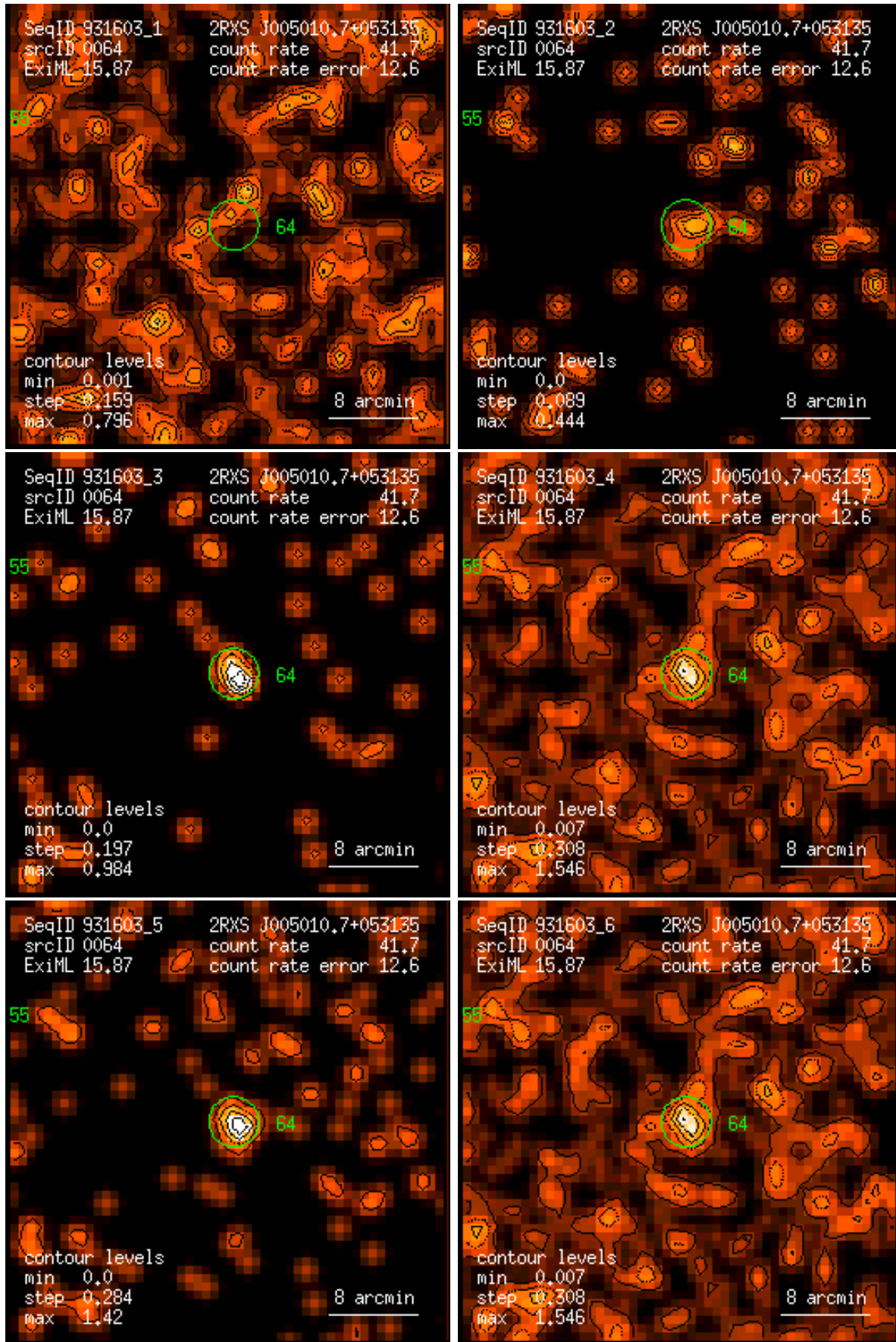
Figure 64: RASS 931603: detection 0064: band rate images, Gaussian filter: (1) PSPC channels 11 – 41, (2) 52 – 90, (3) 91 – 201, (4) 11 – 235, (5) 52 – 201, (6) 11 – 201. Broad band rates in counts/ks. Band rate contour levels in counts/ks/arcmin 2 .
