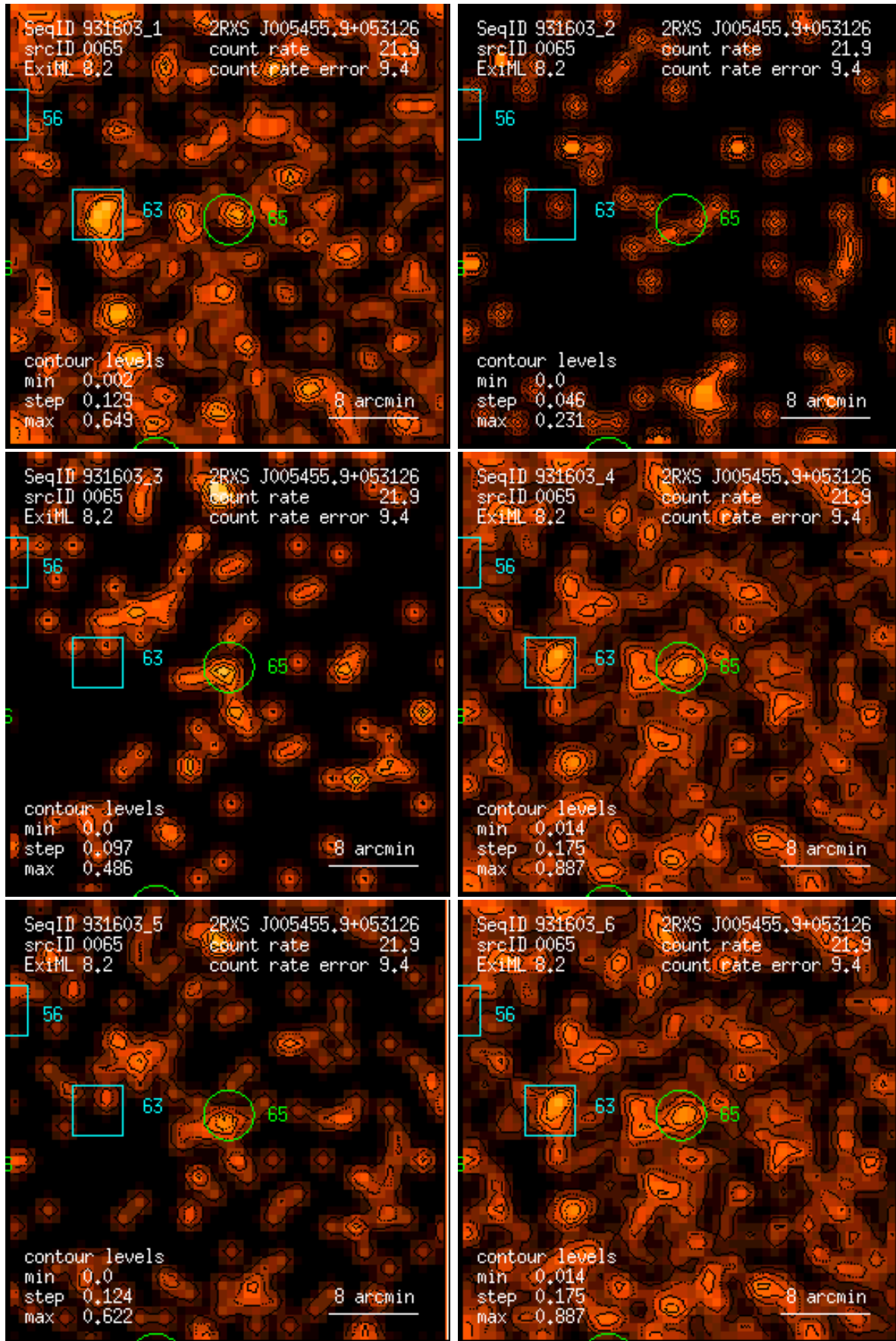
Figure 65: RASS 931603: detection 0065: band rate images, Gaussian filter: (1) PSPC channels 11 – 41, (2) 52 – 90, (3) 91 – 201, (4) 11 – 235, (5) 52 – 201, (6) 11 – 201. Broad band rates in counts/ks. Band rate contour levels in counts/ks/arcmin 2 .
