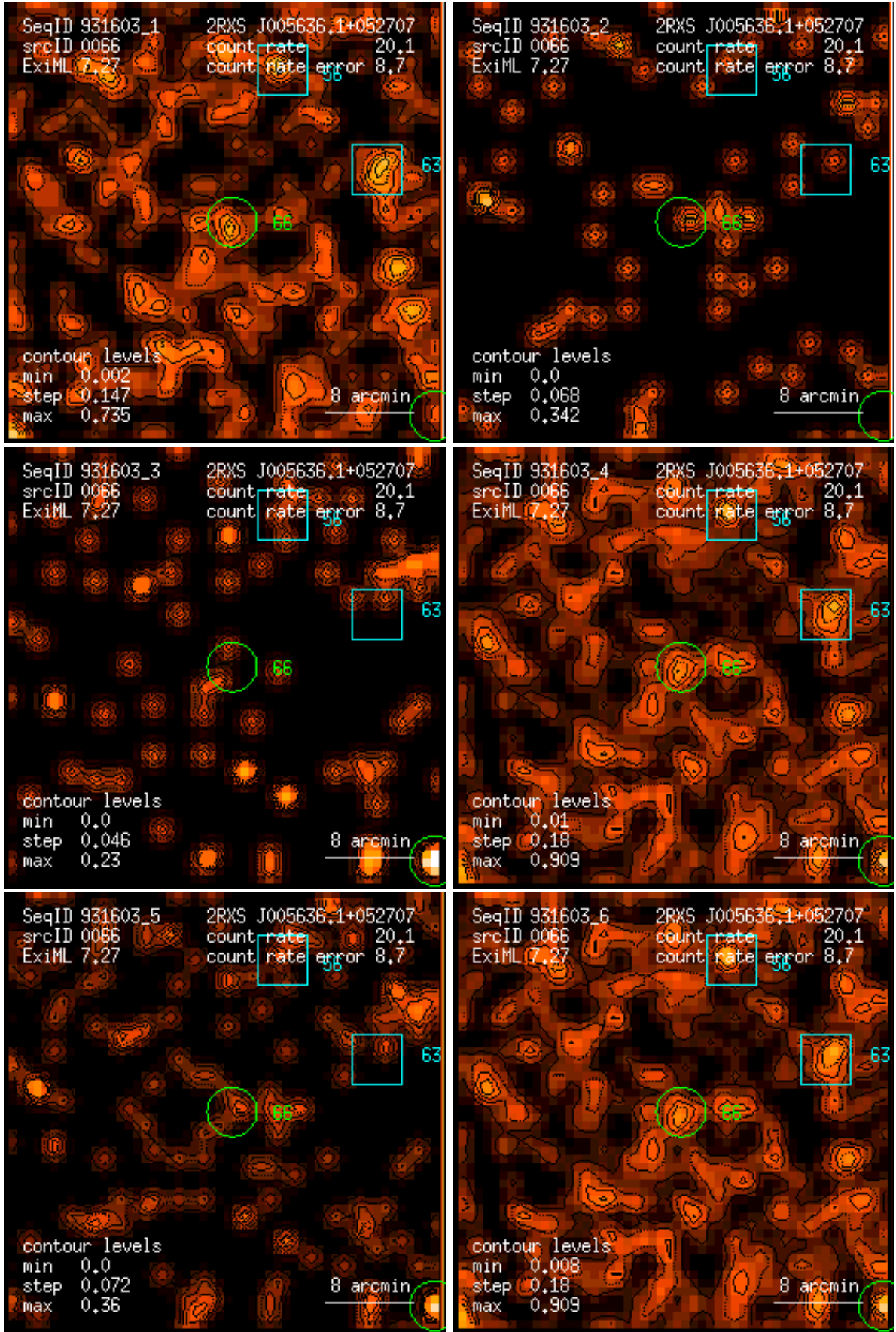
Figure 66: RASS 931603: detection 0066: band rate images, Gaussian filter: (1) PSPC channels 11 – 41, (2) 52 – 90, (3) 91 – 201, (4) 11 – 235, (5) 52 – 201, (6) 11 – 201. Broad band rates in counts/ks. Band rate contour levels in counts/ks/arcmin 2 .
