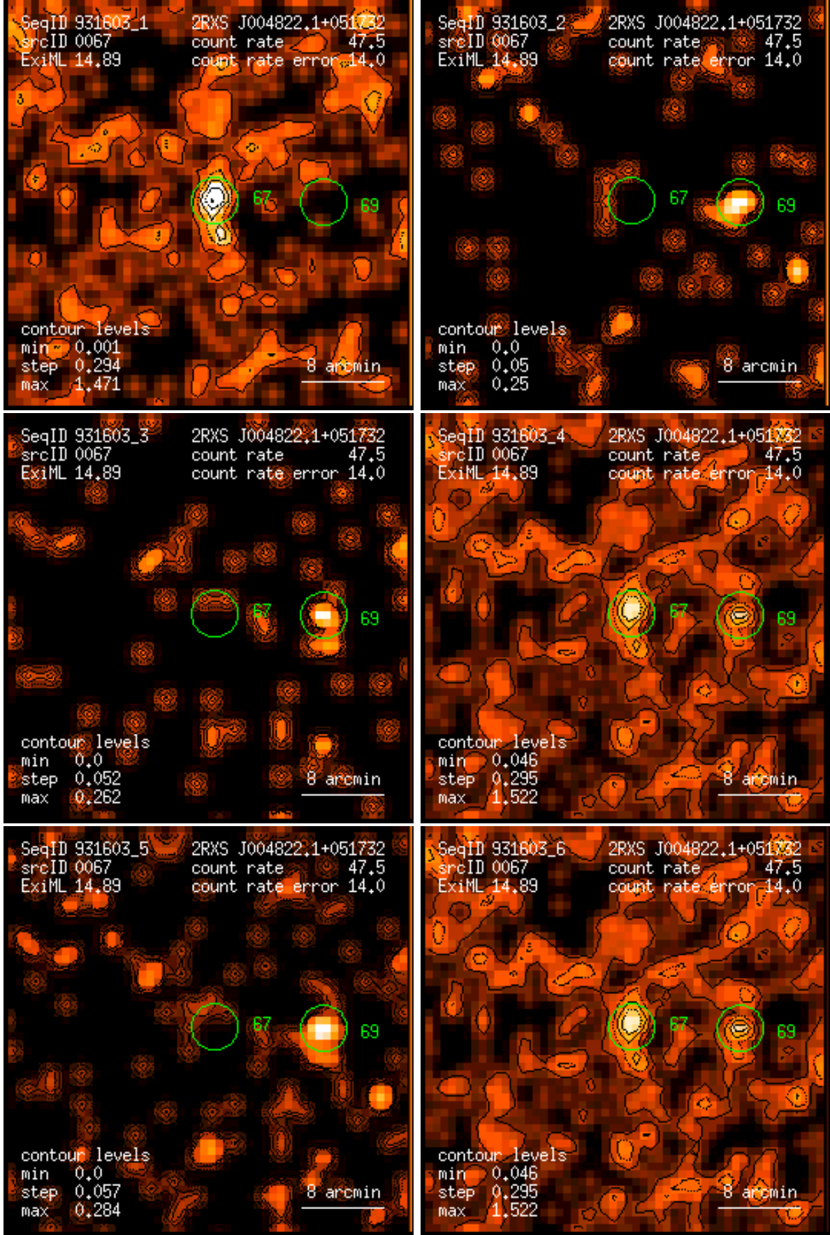
Figure 67: RASS 931603: detection 0067: band rate images, Gaussian filter: (1) PSPC channels 11 – 41, (2) 52 – 90, (3) 91 – 201, (4) 11 – 235, (5) 52 – 201, (6) 11 – 201. Broad band rates in counts/ks. Band rate contour levels in counts/ks/arcmin 2 .
