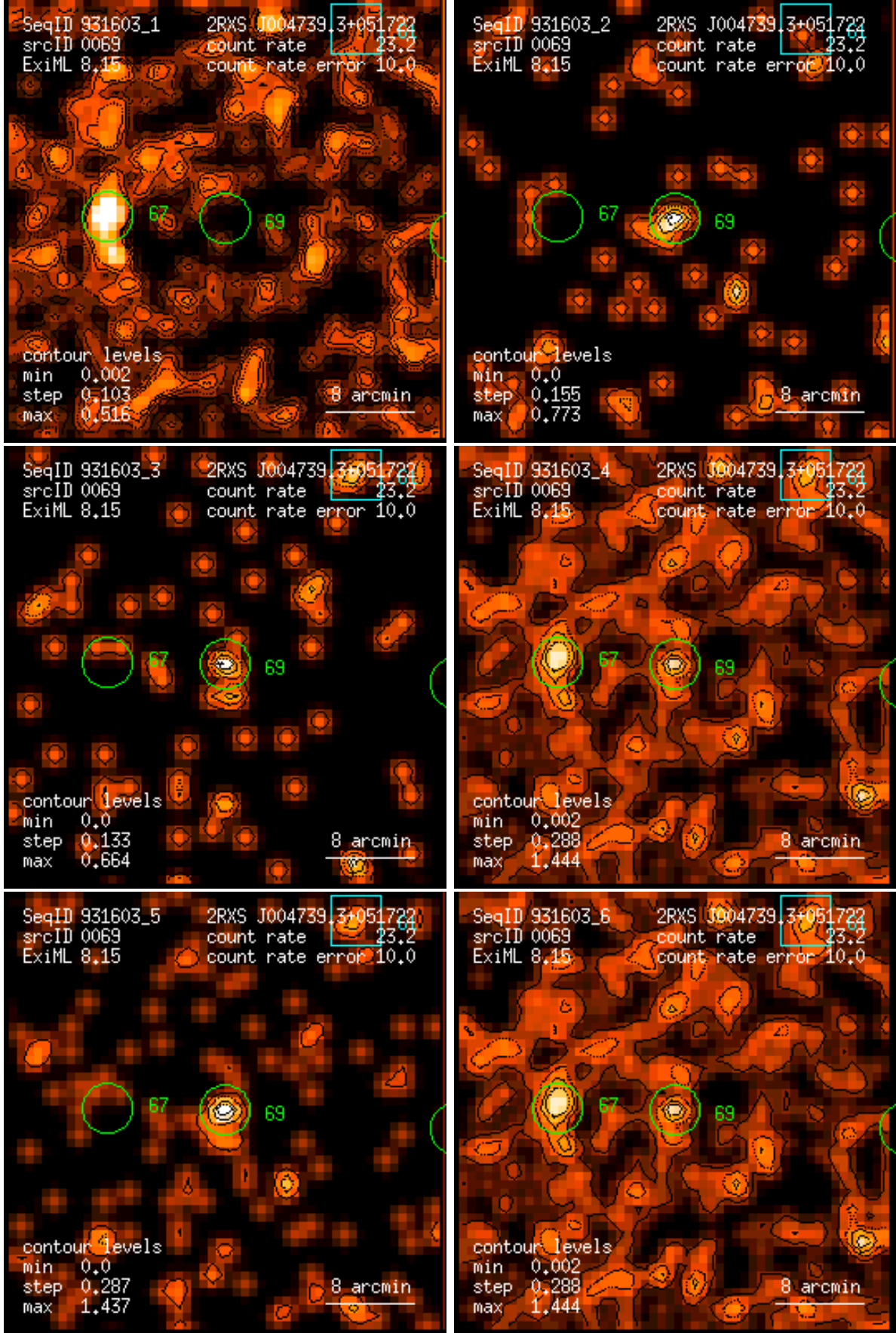
Figure 69: RASS 931603: detection 0069: band rate images, Gaussian filter: (1) PSPC channels 11 – 41, (2) 52 – 90, (3) 91 – 201, (4) 11 – 235, (5) 52 – 201, (6) 11 – 201. Broad band rates in counts/ks. Band rate contour levels in counts/ks/arcmin 2 .
