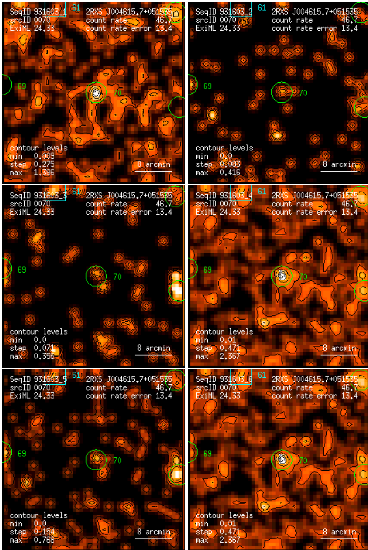
Figure 70: RASS 931603: detection 0070: band rate images, Gaussian filter: (1) PSPC channels 11 – 41, (2) 52 – 90, (3) 91 – 201, (4) 11 – 235, (5) 52 – 201, (6) 11 – 201. Broad band rates in counts/ks. Band rate contour levels in counts/ks/arcmin 2 .
