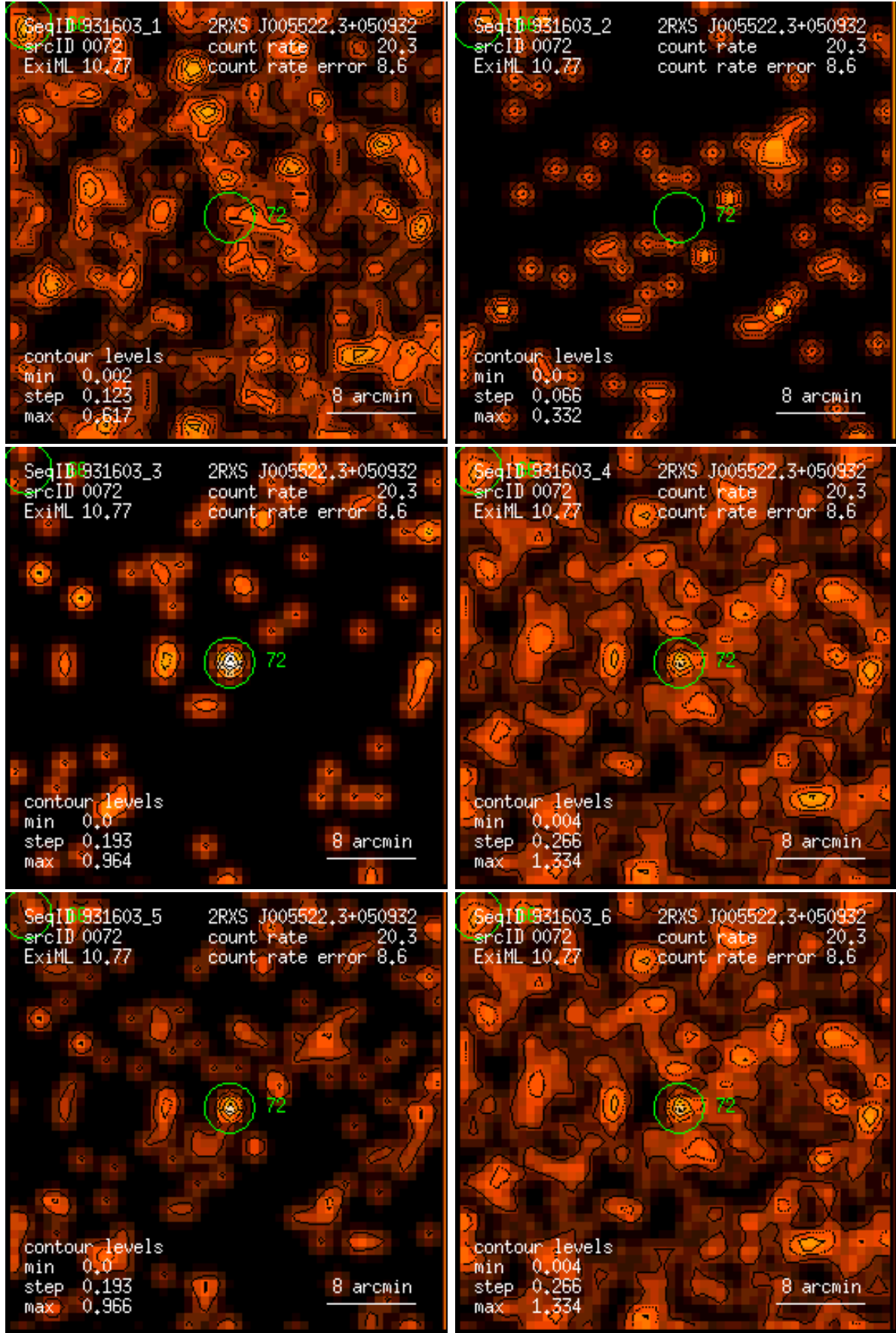
Figure 72: RASS 931603: detection 0072: band rate images, Gaussian filter: (1) PSPC channels 11 – 41, (2) 52 – 90, (3) 91 – 201, (4) 11 – 235, (5) 52 – 201, (6) 11 – 201. Broad band rates in counts/ks. Band rate contour levels in counts/ks/arcmin 2 .
