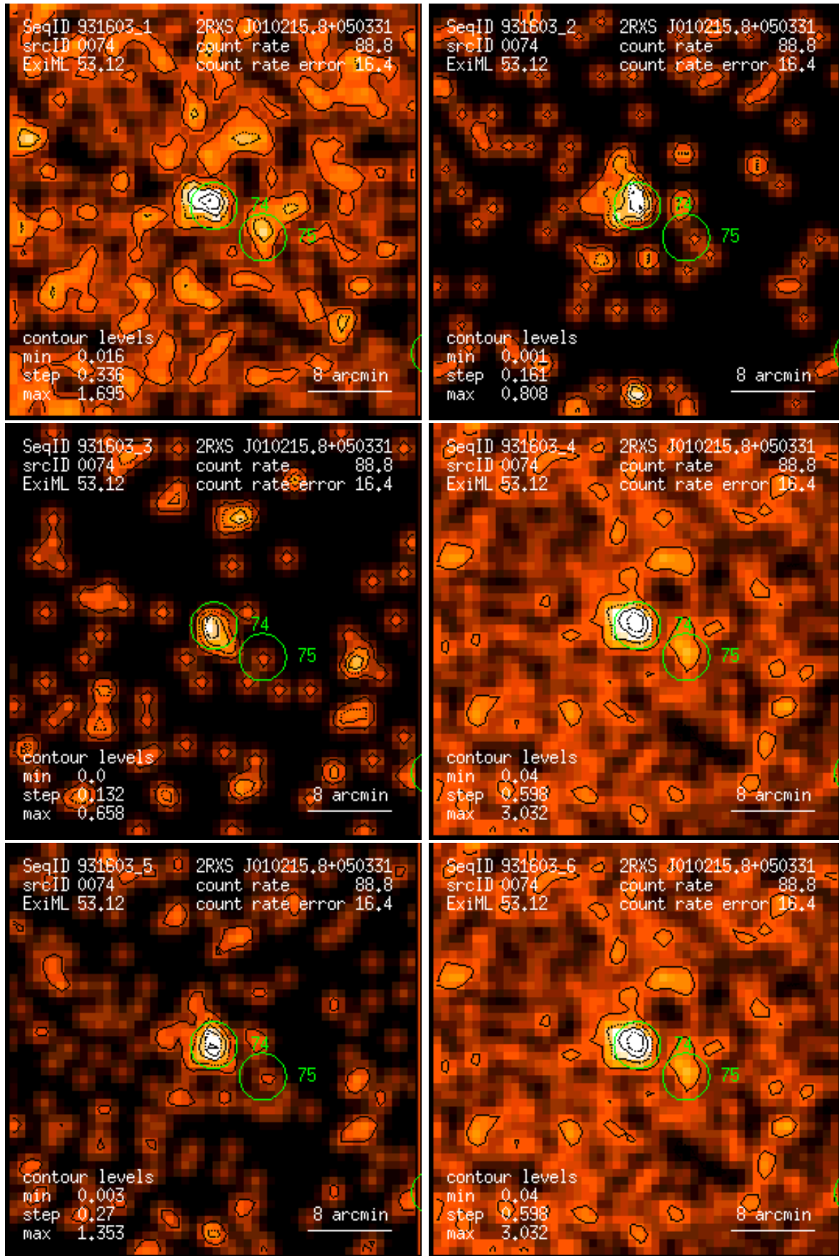
Figure 74: RASS 931603: detection 0074: band rate images, Gaussian filter: (1) PSPC channels 11 – 41, (2) 52 – 90, (3) 91 – 201, (4) 11 – 235, (5) 52 – 201, (6) 11 – 201. Broad band rates in counts/ks. Band rate contour levels in counts/ks/arcmin 2 .
