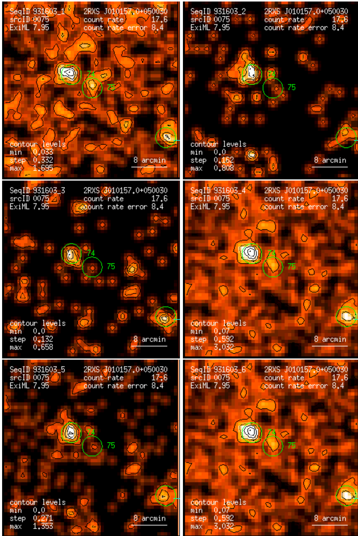
Figure 75: RASS 931603: detection 0075: band rate images, Gaussian filter: (1) PSPC channels 11 – 41, (2) 52 – 90, (3) 91 – 201, (4) 11 – 235, (5) 52 – 201, (6) 11 – 201. Broad band rates in counts/ks. Band rate contour levels in counts/ks/arcmin 2 .
