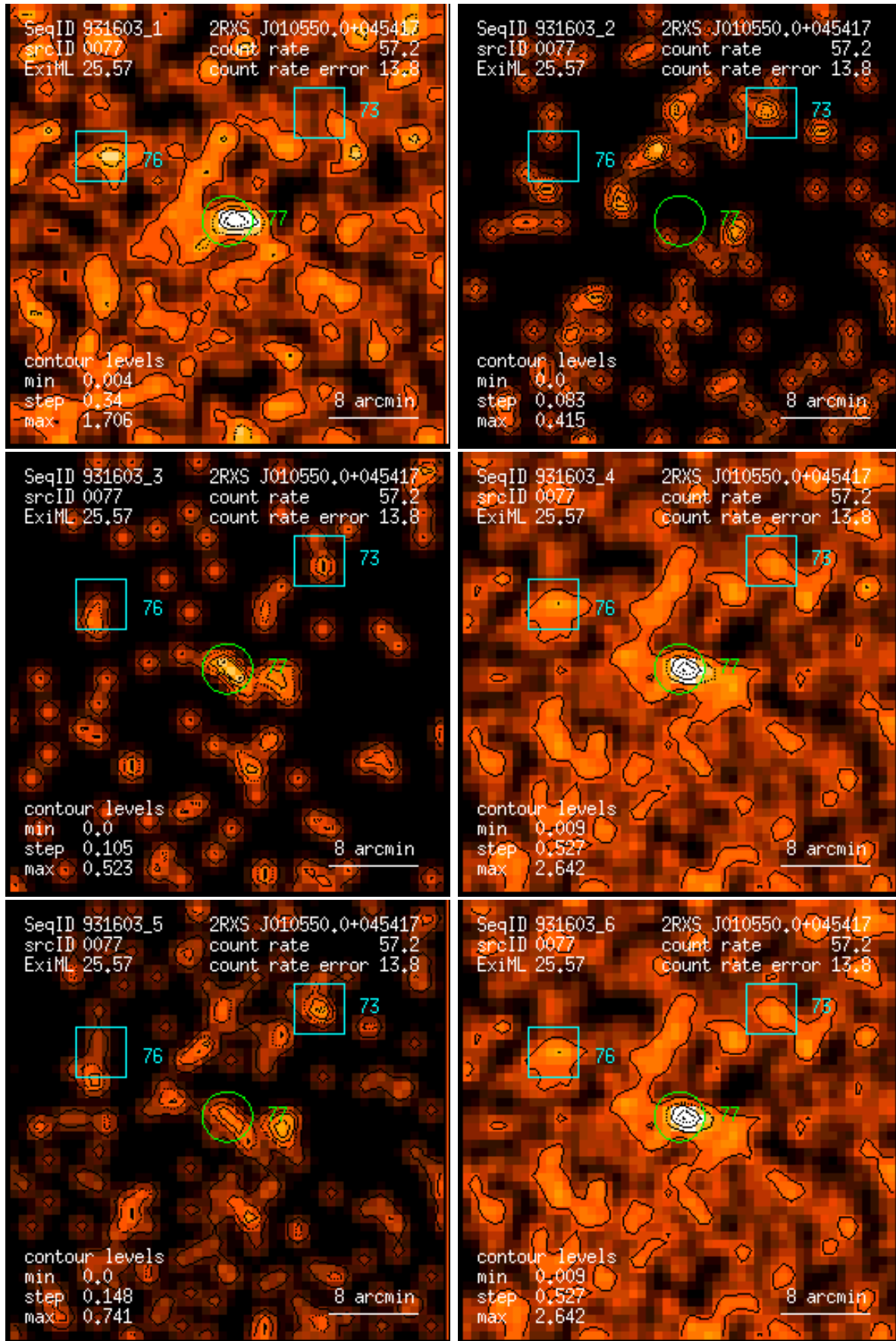
Figure 77: RASS 931603: detection 0077: band rate images, Gaussian filter: (1) PSPC channels 11 – 41, (2) 52 – 90, (3) 91 – 201, (4) 11 – 235, (5) 52 – 201, (6) 11 – 201. Broad band rates in counts/ks. Band rate contour levels in counts/ks/arcmin 2 .
