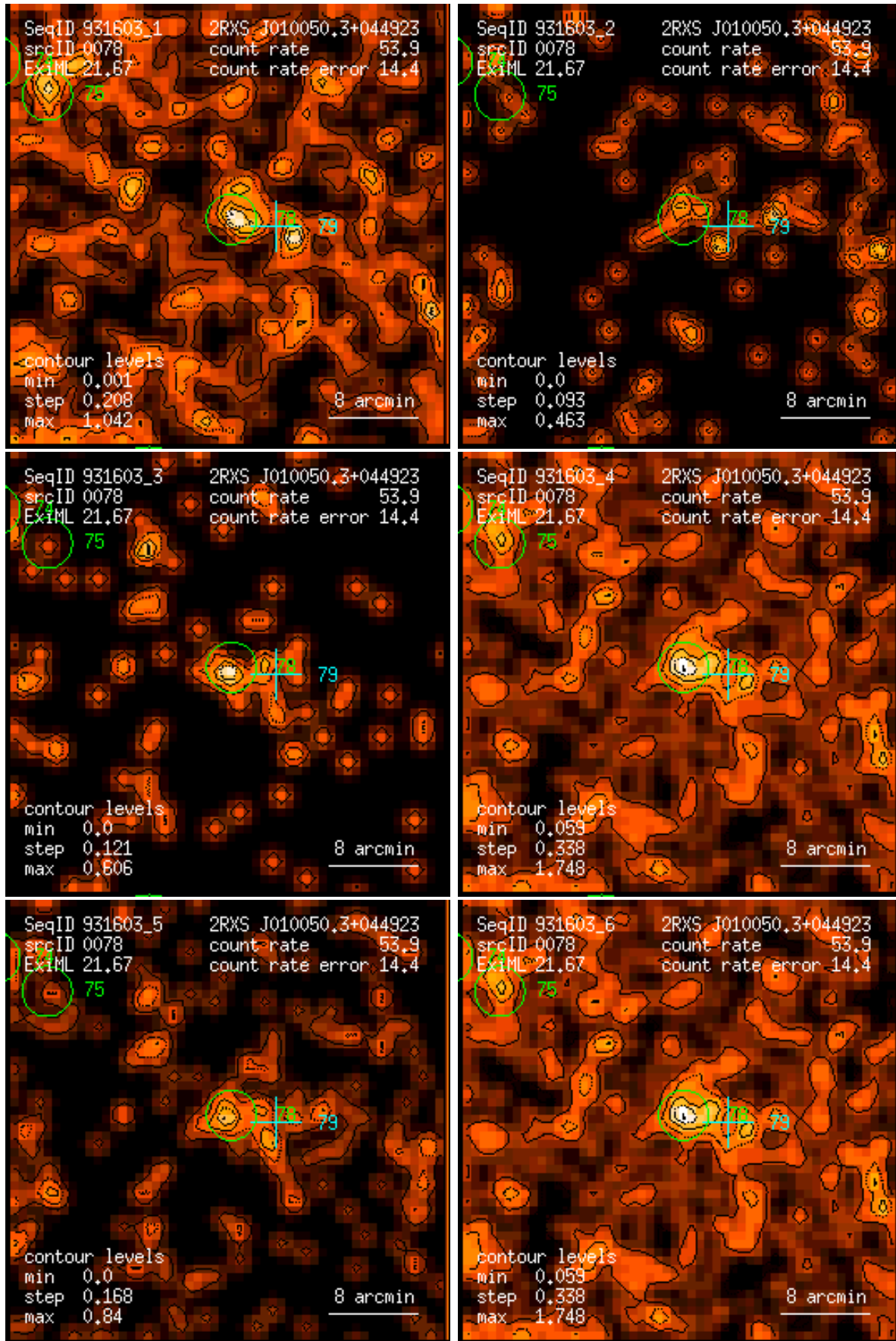
Figure 78: RASS 931603: detection 0078: band rate images, Gaussian filter: (1) PSPC channels 11 – 41, (2) 52 – 90, (3) 91 – 201, (4) 11 – 235, (5) 52 – 201, (6) 11 – 201. Broad band rates in counts/ks. Band rate contour levels in counts/ks/arcmin 2 .
