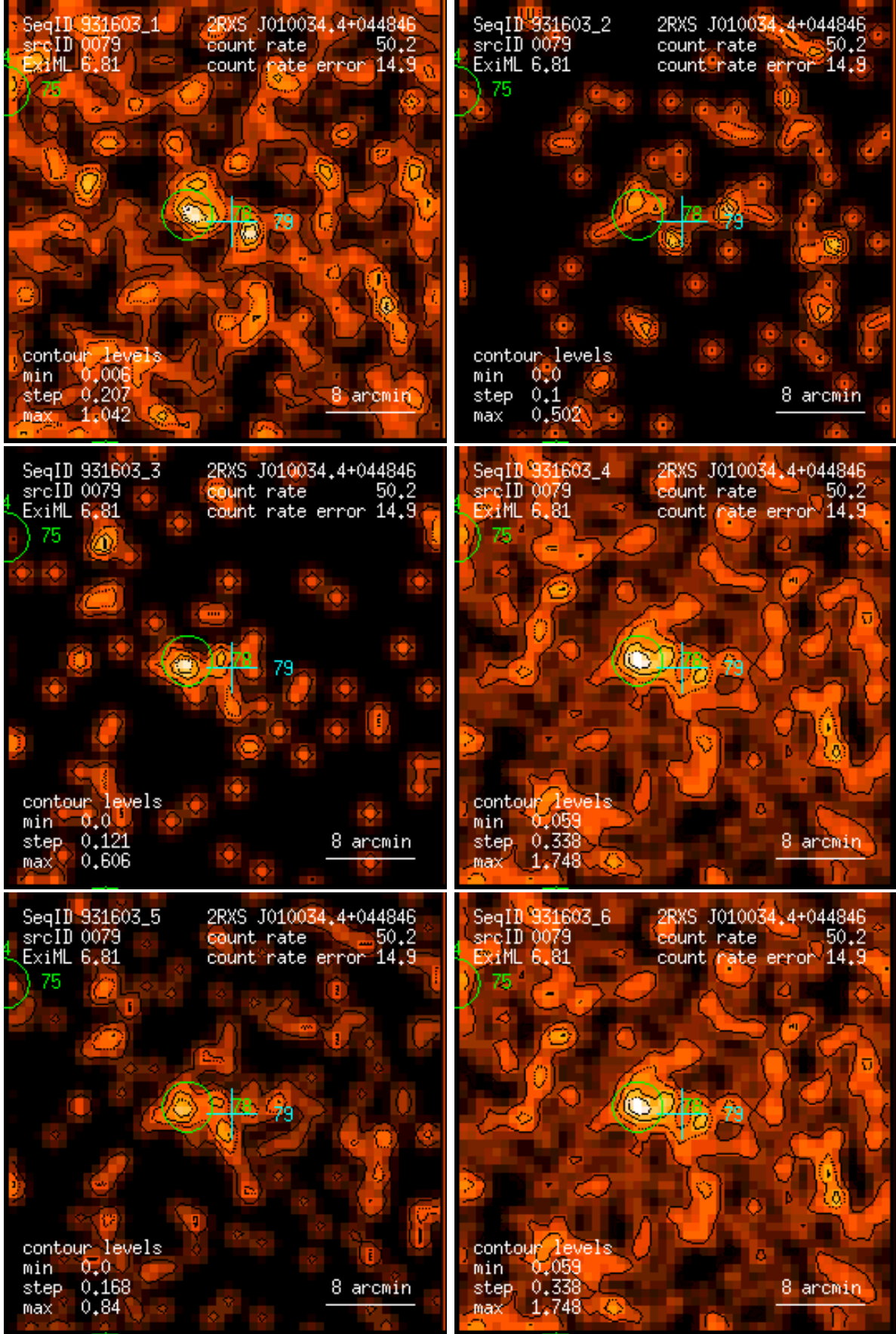
Figure 79: RASS 931603: detection 0079: band rate images, Gaussian filter: (1) PSPC channels 11 – 41, (2) 52 – 90, (3) 91 – 201, (4) 11 – 235, (5) 52 – 201, (6) 11 – 201. Broad band rates in counts/ks. Band rate contour levels in counts/ks/arcmin 2 .
