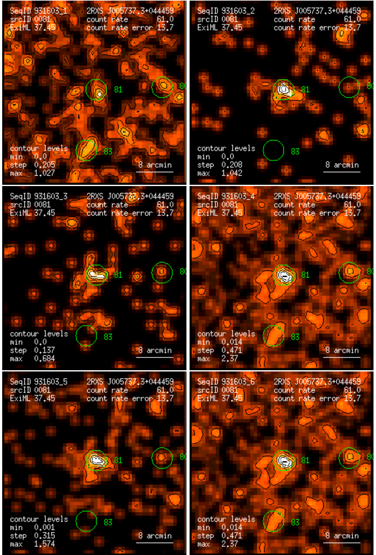
Figure 81: RASS 931603: detection 0081: band rate images, Gaussian filter: (1) PSPC channels 11 – 41, (2) 52 – 90, (3) 91 – 201, (4) 11 – 235, (5) 52 – 201, (6) 11 – 201. Broad band rates in counts/ks. Band rate contour levels in counts/ks/arcmin 2 .
