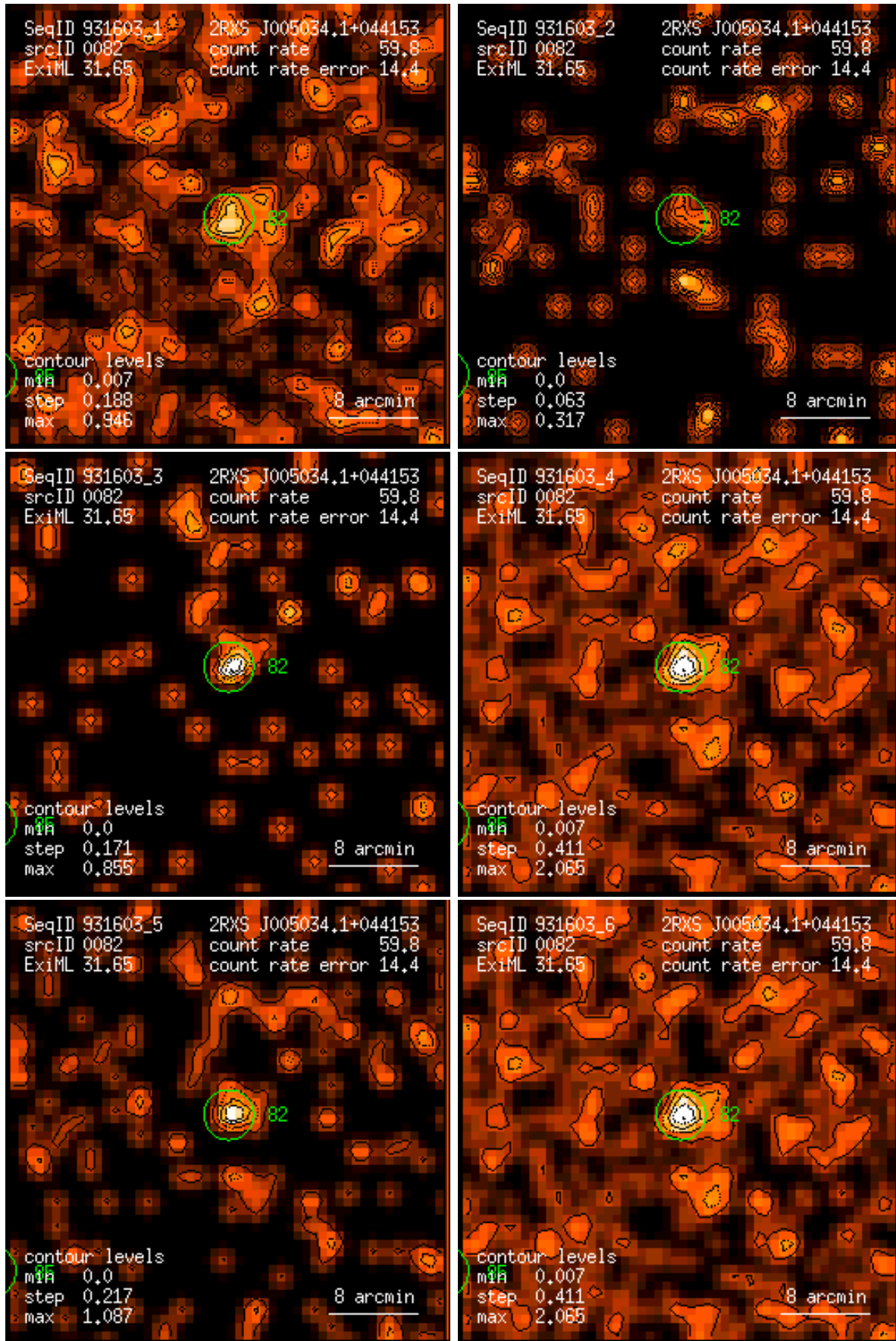
Figure 82: RASS 931603: detection 0082: band rate images, Gaussian filter: (1) PSPC channels 11 – 41, (2) 52 – 90, (3) 91 – 201, (4) 11 – 235, (5) 52 – 201, (6) 11 – 201. Broad band rates in counts/ks. Band rate contour levels in counts/ks/arcmin 2 .
