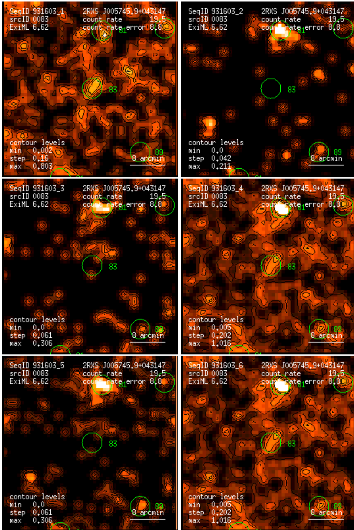
Figure 83: RASS 931603: detection 0083: band rate images, Gaussian filter: (1) PSPC channels 11 – 41, (2) 52 – 90, (3) 91 – 201, (4) 11 – 235, (5) 52 – 201, (6) 11 – 201. Broad band rates in counts/ks. Band rate contour levels in counts/ks/arcmin 2 .
