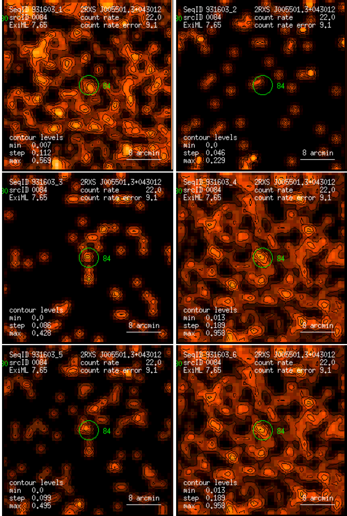
Figure 84: RASS 931603: detection 0084: band rate images, Gaussian filter: (1) PSPC channels 11 – 41, (2) 52 – 90, (3) 91 – 201, (4) 11 – 235, (5) 52 – 201, (6) 11 – 201. Broad band rates in counts/ks. Band rate contour levels in counts/ks/arcmin 2 .
