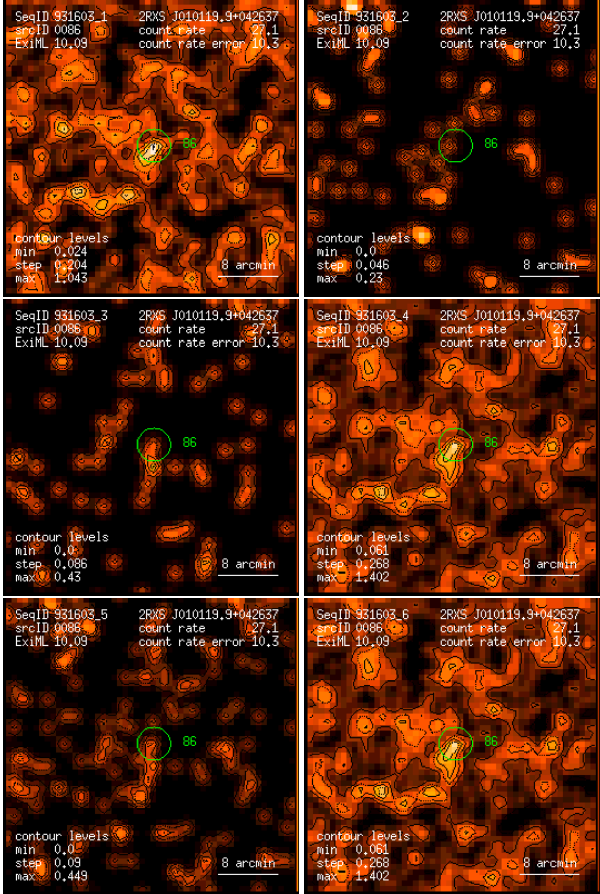
Figure 86: RASS 931603: detection 0086: band rate images, Gaussian filter: (1) PSPC channels 11 – 41, (2) 52 – 90, (3) 91 – 201, (4) 11 – 235, (5) 52 – 201, (6) 11 – 201. Broad band rates in counts/ks. Band rate contour levels in counts/ks/arcmin 2 .
