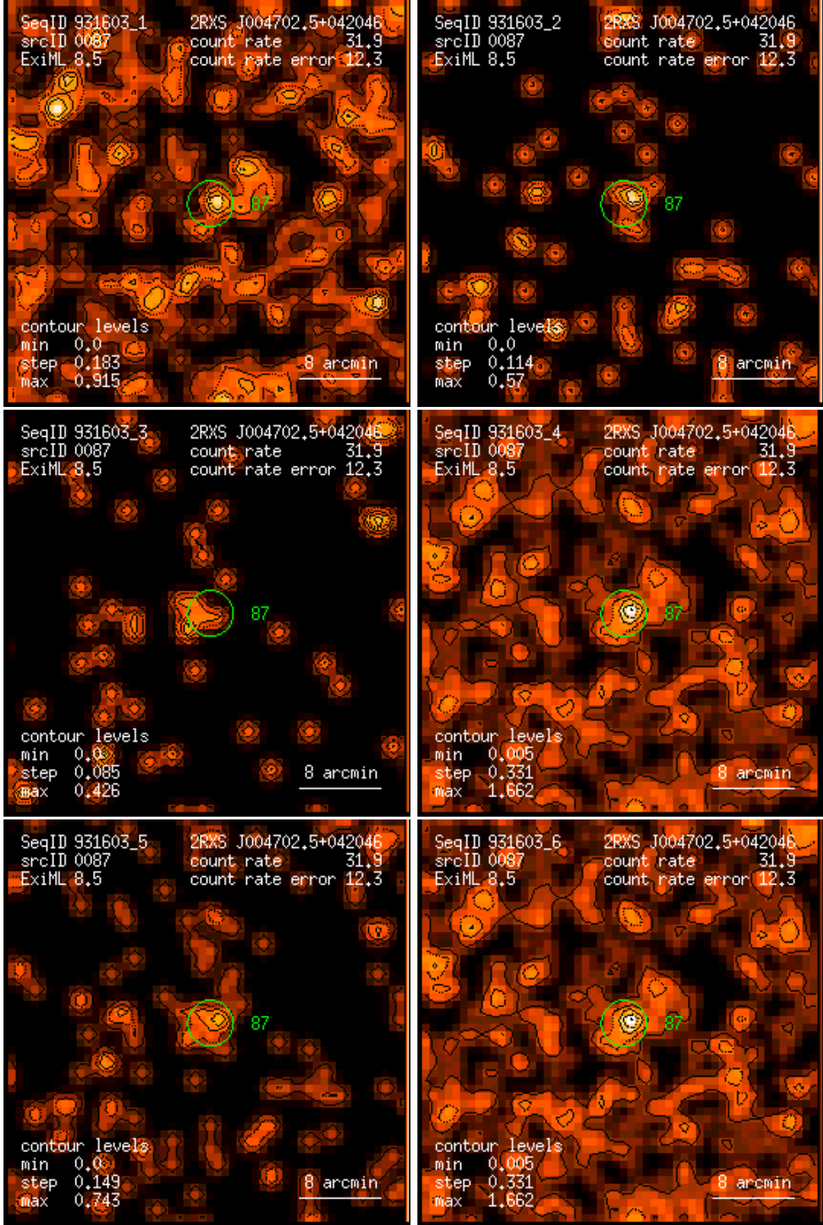
Figure 87: RASS 931603: detection 0087: band rate images, Gaussian filter: (1) PSPC channels 11 – 41, (2) 52 – 90, (3) 91 – 201, (4) 11 – 235, (5) 52 – 201, (6) 11 – 201. Broad band rates in counts/ks. Band rate contour levels in counts/ks/arcmin 2 .
