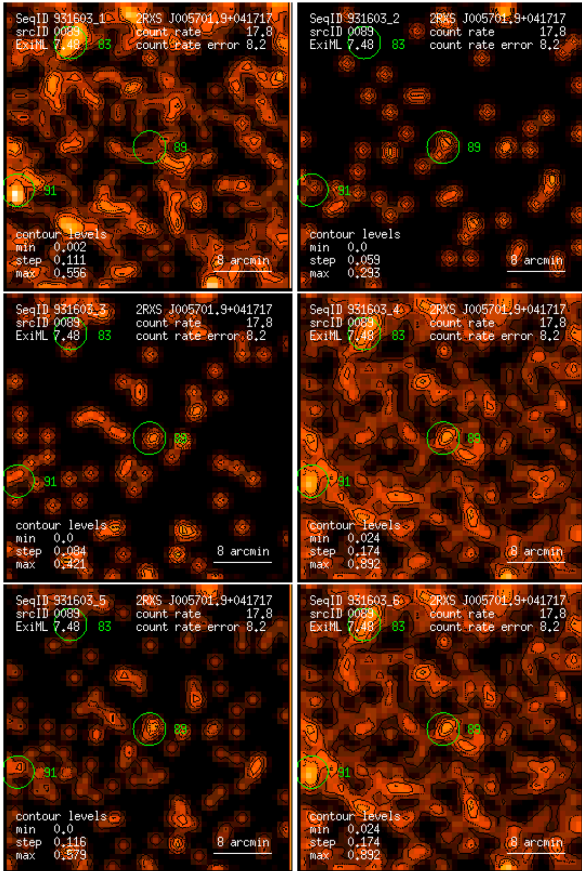
Figure 89: RASS 931603: detection 0089: band rate images, Gaussian filter: (1) PSPC channels 11 – 41, (2) 52 – 90, (3) 91 – 201, (4) 11 – 235, (5) 52 – 201, (6) 11 – 201. Broad band rates in counts/ks. Band rate contour levels in counts/ks/arcmin 2 .
