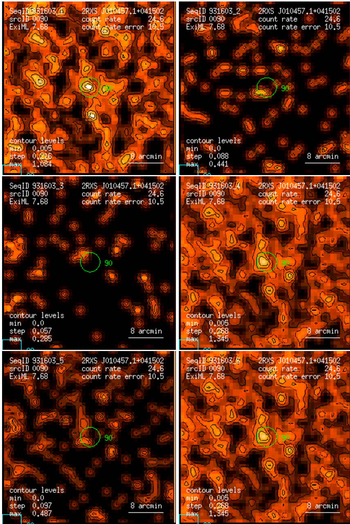
Figure 90: RASS 931603: detection 0090: band rate images, Gaussian filter: (1) PSPC channels 11 – 41, (2) 52 – 90, (3) 91 – 201, (4) 11 – 235, (5) 52 – 201, (6) 11 – 201. Broad band rates in counts/ks. Band rate contour levels in counts/ks/arcmin 2 .
