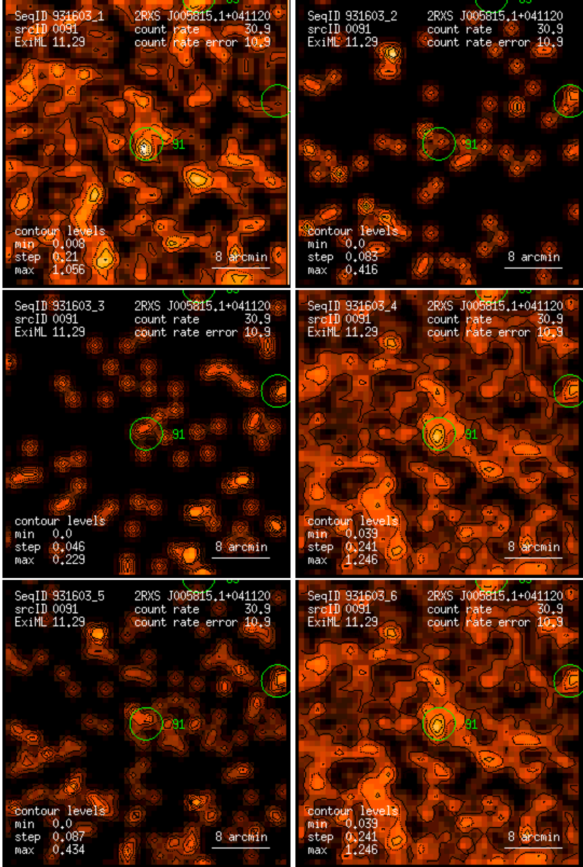
Figure 91: RASS 931603: detection 0091: band rate images, Gaussian filter: (1) PSPC channels 11 – 41, (2) 52 – 90, (3) 91 – 201, (4) 11 – 235, (5) 52 – 201, (6) 11 – 201. Broad band rates in counts/ks. Band rate contour levels in counts/ks/arcmin 2 .
