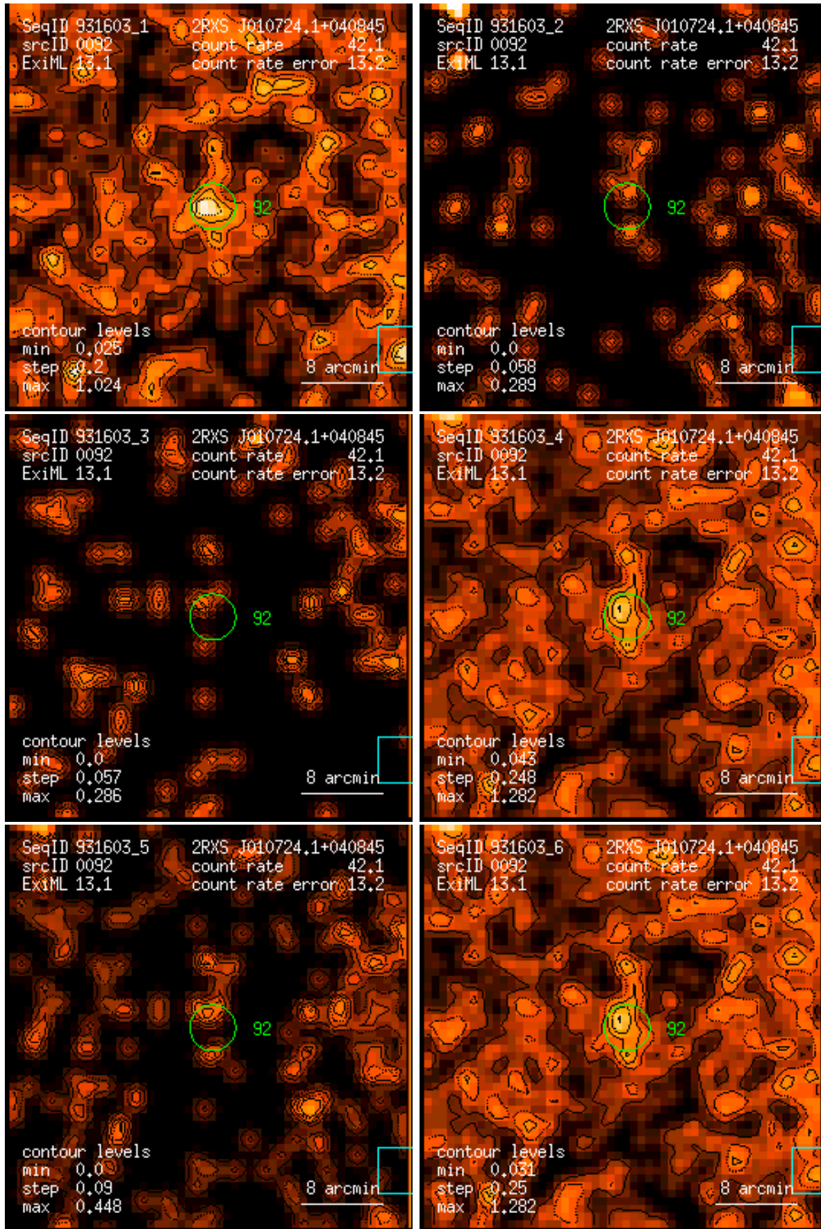
Figure 92: RASS 931603: detection 0092: band rate images, Gaussian filter: (1) PSPC channels 11 – 41, (2) 52 – 90, (3) 91 – 201, (4) 11 – 235, (5) 52 – 201, (6) 11 – 201. Broad band rates in counts/ks. Band rate contour levels in counts/ks/arcmin 2 .
