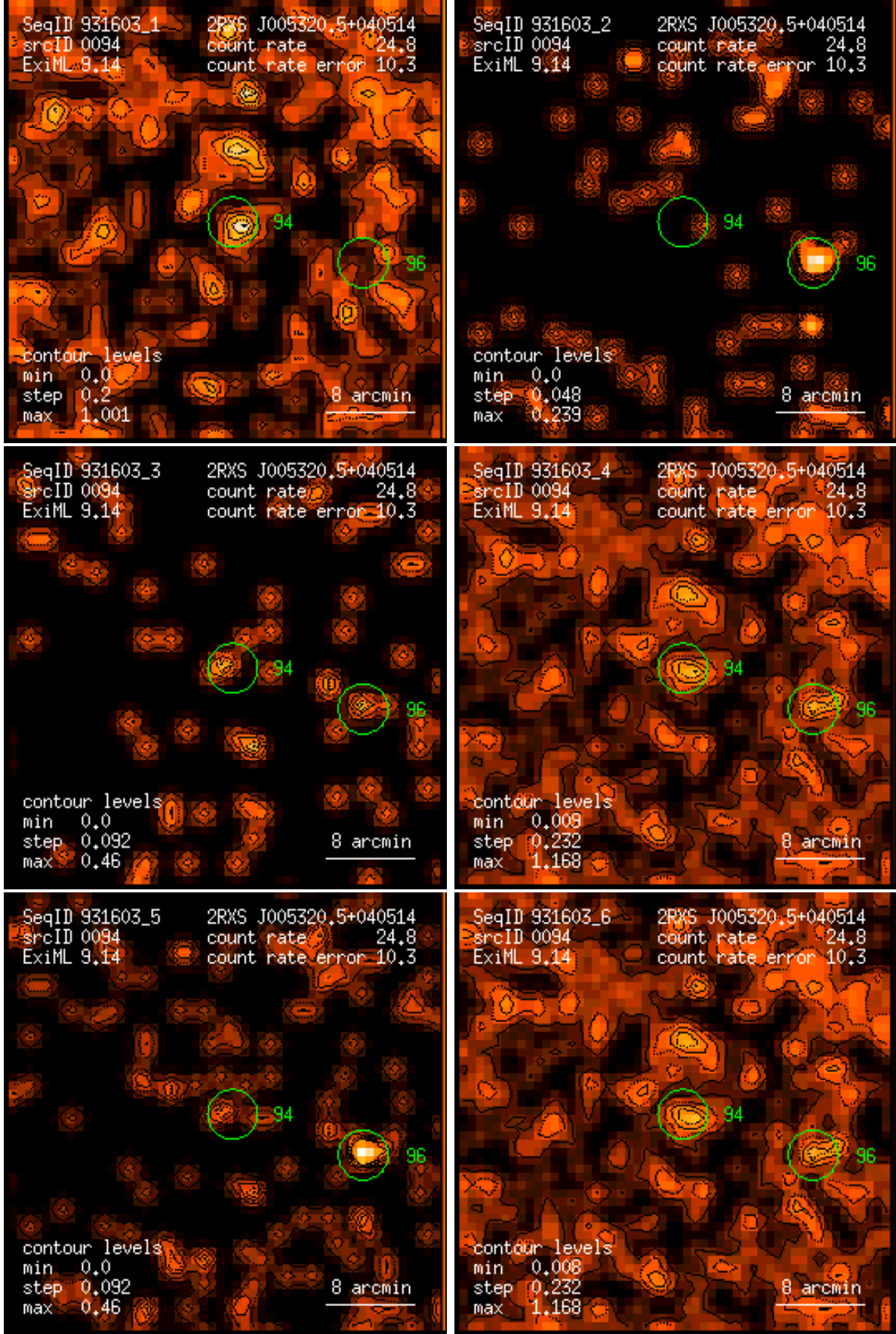
Figure 94: RASS 931603: detection 0094: band rate images, Gaussian filter: (1) PSPC channels 11 – 41, (2) 52 – 90, (3) 91 – 201, (4) 11 – 235, (5) 52 – 201, (6) 11 – 201. Broad band rates in counts/ks. Band rate contour levels in counts/ks/arcmin 2 .
