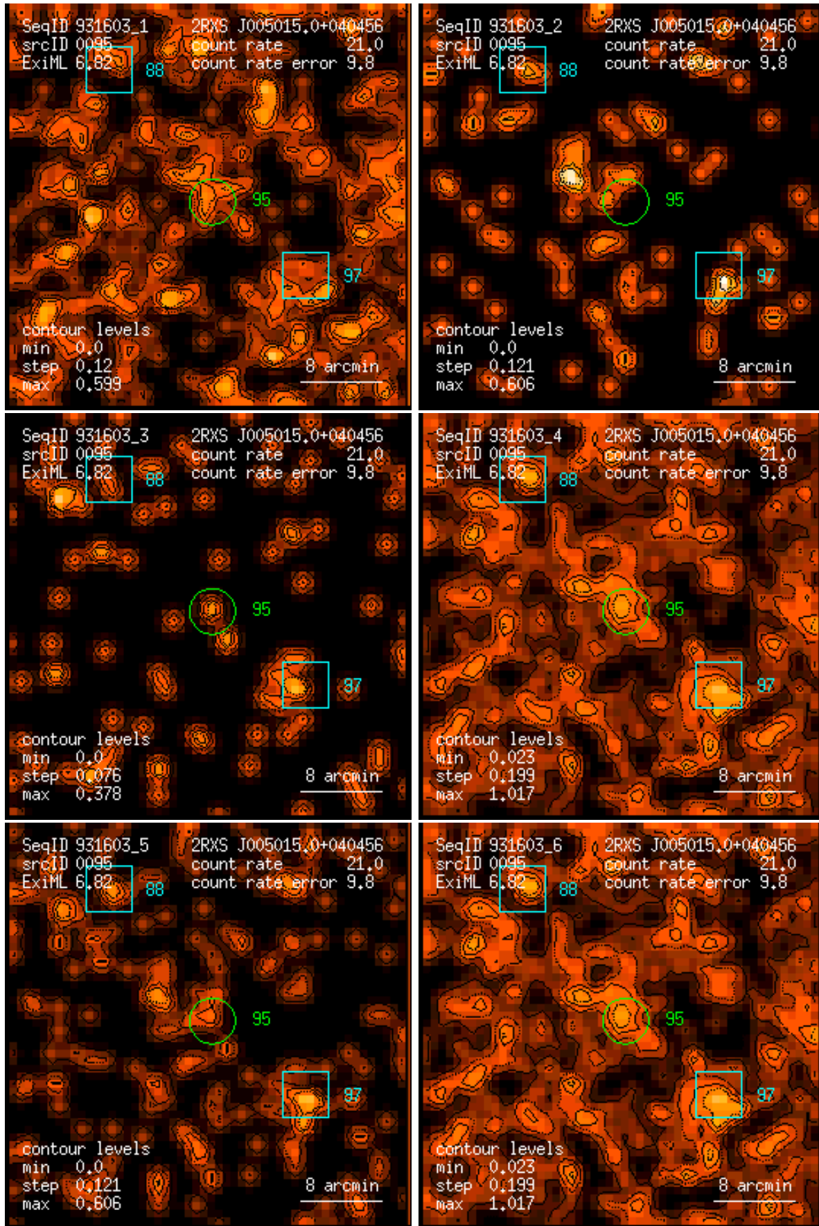
Figure 95: RASS 931603: detection 0095: band rate images, Gaussian filter: (1) PSPC channels 11 – 41, (2) 52 – 90, (3) 91 – 201, (4) 11 – 235, (5) 52 – 201, (6) 11 – 201. Broad band rates in counts/ks. Band rate contour levels in counts/ks/arcmin 2 .
