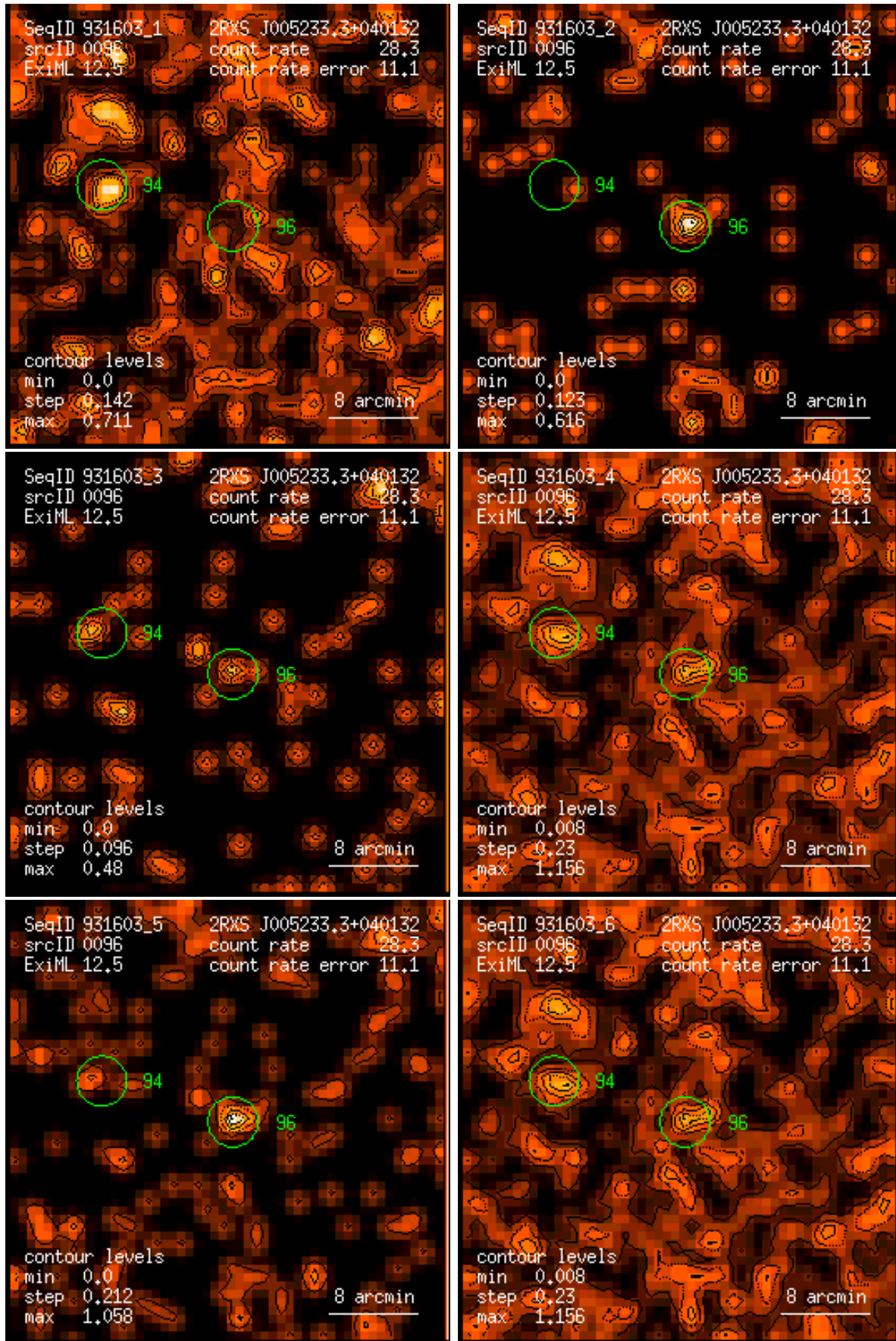
Figure 96: RASS 931603: detection 0096: band rate images, Gaussian filter: (1) PSPC channels 11 – 41, (2) 52 – 90, (3) 91 – 201, (4) 11 – 235, (5) 52 – 201, (6) 11 – 201. Broad band rates in counts/ks. Band rate contour levels in counts/ks/arcmin 2 .
