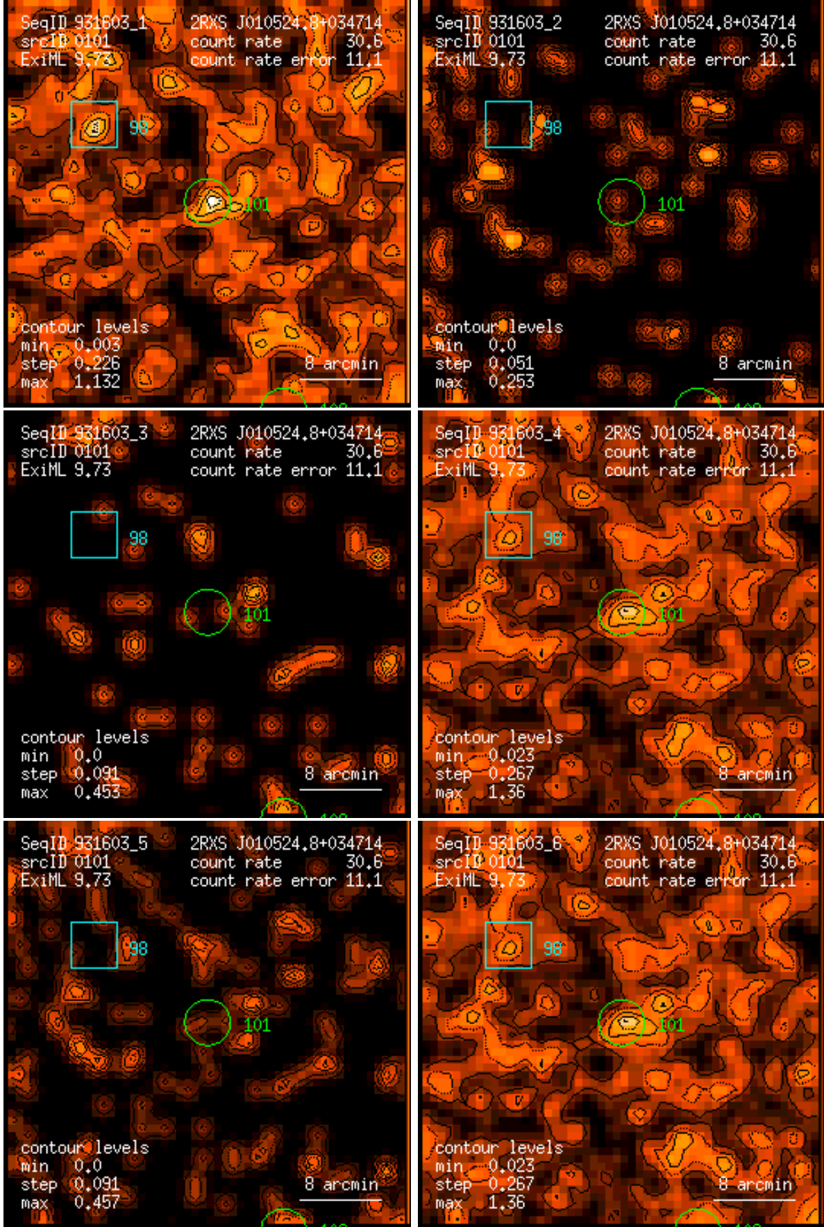
Figure 101: RASS 931603: detection 0101: band rate images, Gaussian filter: (1) PSPC channels 11 – 41, (2) 52 – 90, (3) 91 – 201, (4) 11 – 235, (5) 52 – 201, (6) 11 – 201. Broad band rates in counts/ks. Band rate contour levels in counts/ks/arcmin 2 .
