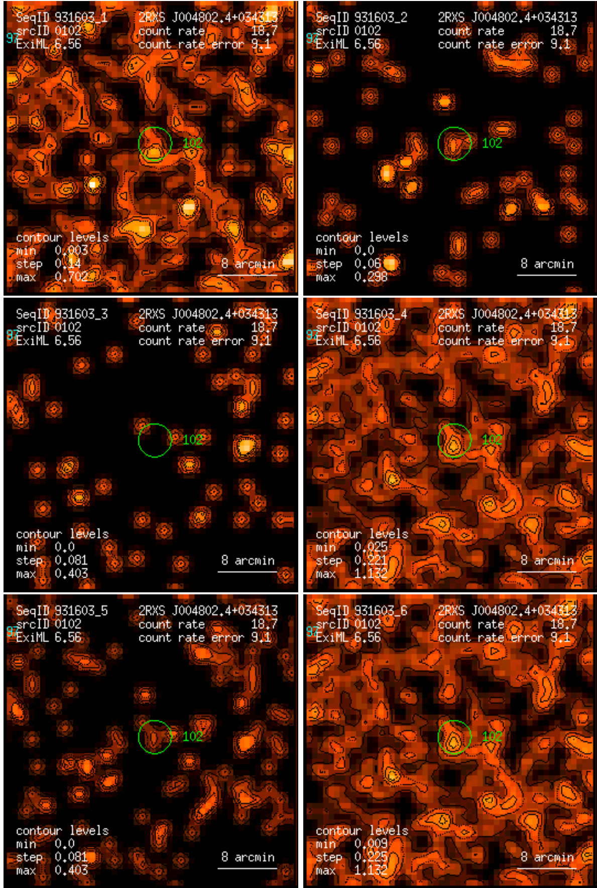
Figure 102: RASS 931603: detection 0102: band rate images, Gaussian filter: (1) PSPC channels 11 – 41, (2) 52 – 90, (3) 91 – 201, (4) 11 – 235, (5) 52 – 201, (6) 11 – 201. Broad band rates in counts/ks. Band rate contour levels in counts/ks/arcmin 2 .
