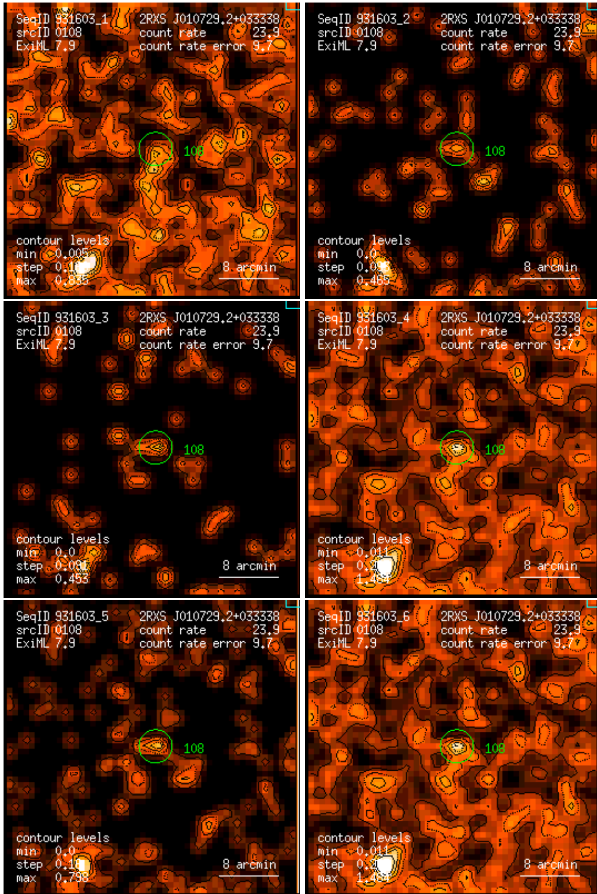
Figure 108: RASS 931603: detection 0108: band rate images, Gaussian filter: (1) PSPC channels 11 – 41, (2) 52 – 90, (3) 91 – 201, (4) 11 – 235, (5) 52 – 201, (6) 11 – 201. Broad band rates in counts/ks. Band rate contour levels in counts/ks/arcmin 2 .
