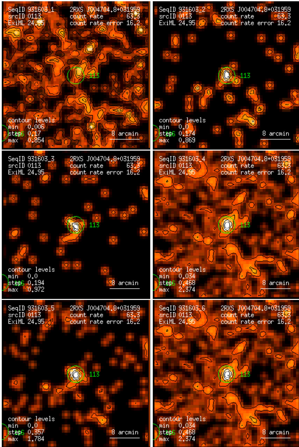
Figure 113: RASS 931603: detection 0113: band rate images, Gaussian filter: (1) PSPC channels 11 – 41, (2) 52 – 90, (3) 91 – 201, (4) 11 – 235, (5) 52 – 201, (6) 11 – 201. Broad band rates in counts/ks. Band rate contour levels in counts/ks/arcmin 2 .
