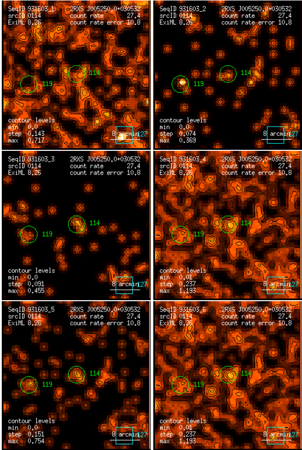
Figure 114: RASS 931603: detection 0114: band rate images, Gaussian filter: (1) PSPC channels 11 – 41, (2) 52 – 90, (3) 91 – 201, (4) 11 – 235, (5) 52 – 201, (6) 11 – 201. Broad band rates in counts/ks. Band rate contour levels in counts/ks/arcmin 2 .
