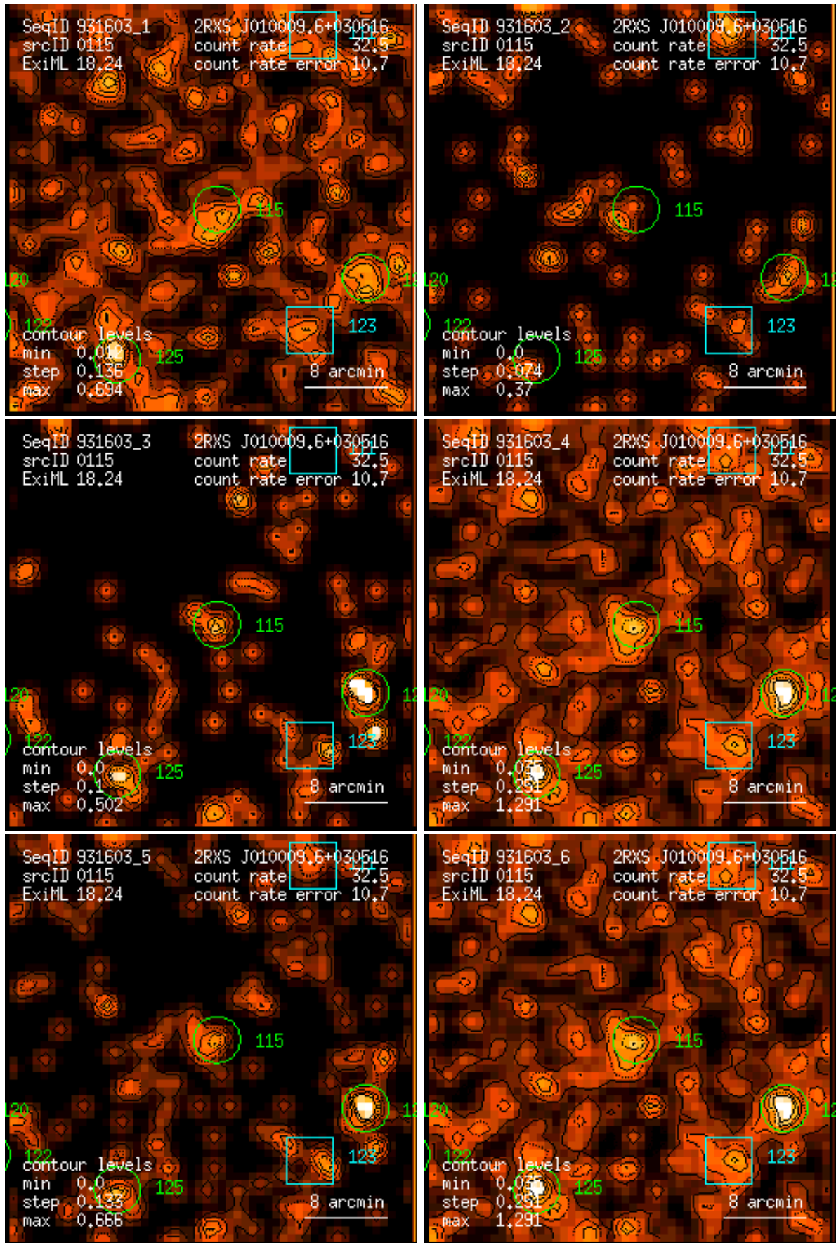
Figure 115: RASS 931603: detection 0115: band rate images, Gaussian filter: (1) PSPC channels 11 – 41, (2) 52 – 90, (3) 91 – 201, (4) 11 – 235, (5) 52 – 201, (6) 11 – 201. Broad band rates in counts/ks. Band rate contour levels in counts/ks/arcmin 2 .
