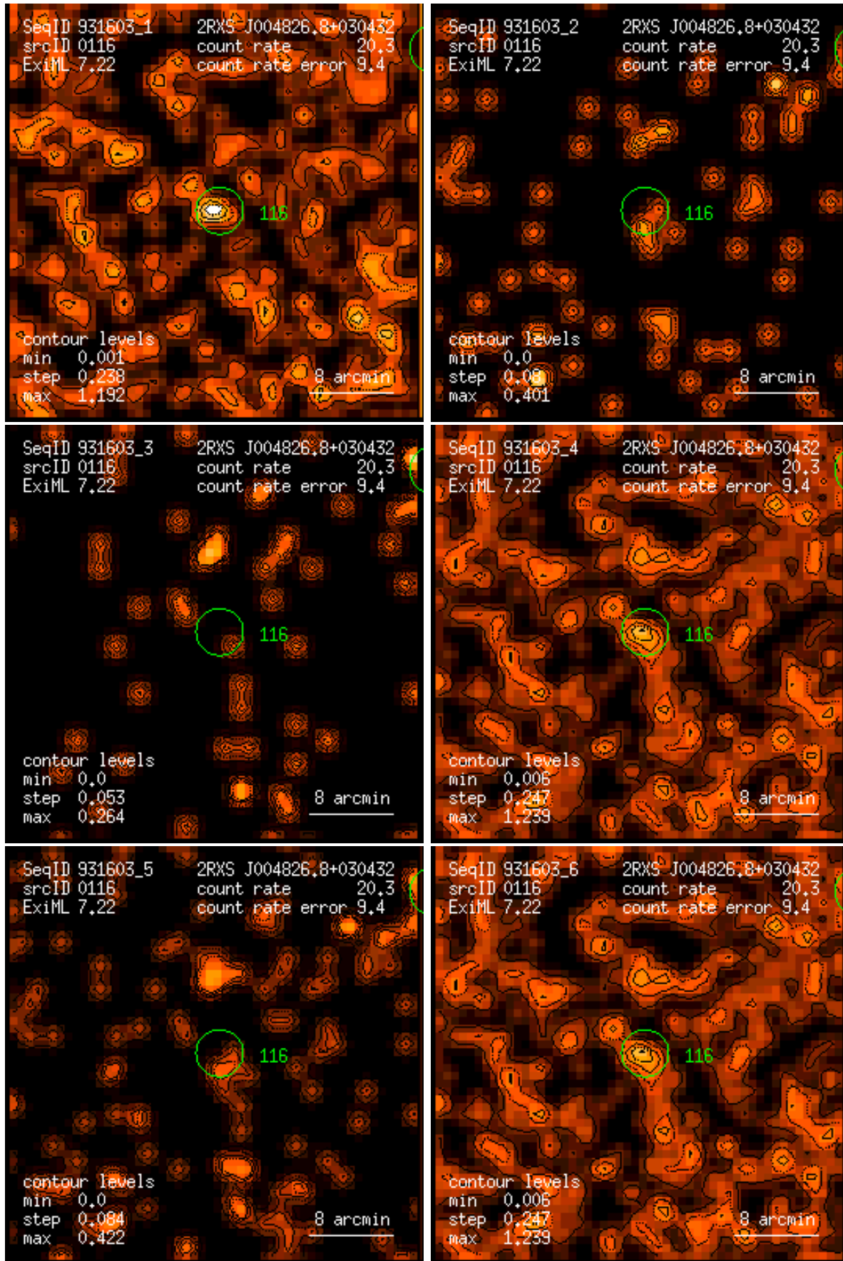
Figure 116: RASS 931603: detection 0116: band rate images, Gaussian filter: (1) PSPC channels 11 – 41, (2) 52 – 90, (3) 91 – 201, (4) 11 – 235, (5) 52 – 201, (6) 11 – 201. Broad band rates in counts/ks. Band rate contour levels in counts/ks/arcmin 2 .
