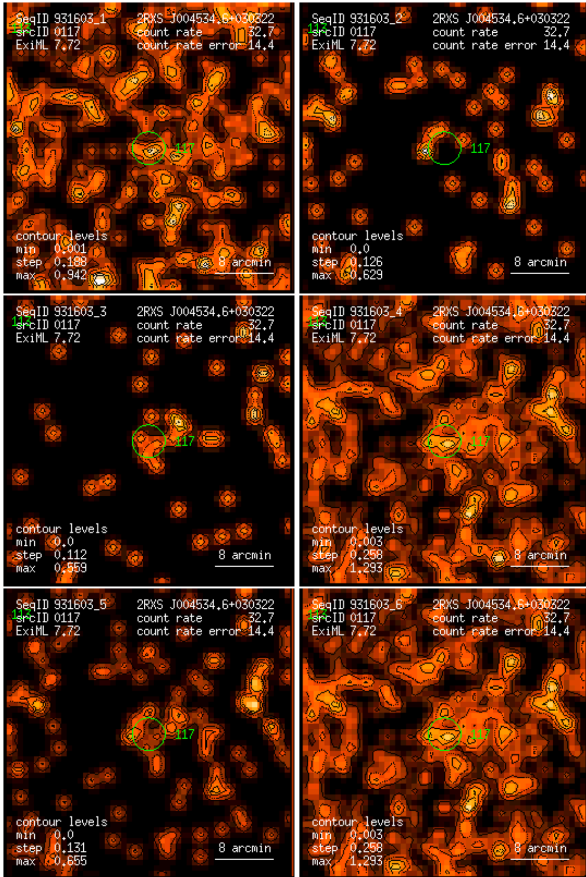
Figure 117: RASS 931603: detection 0117: band rate images, Gaussian filter: (1) PSPC channels 11 – 41, (2) 52 – 90, (3) 91 – 201, (4) 11 – 235, (5) 52 – 201, (6) 11 – 201. Broad band rates in counts/ks. Band rate contour levels in counts/ks/arcmin 2 .
