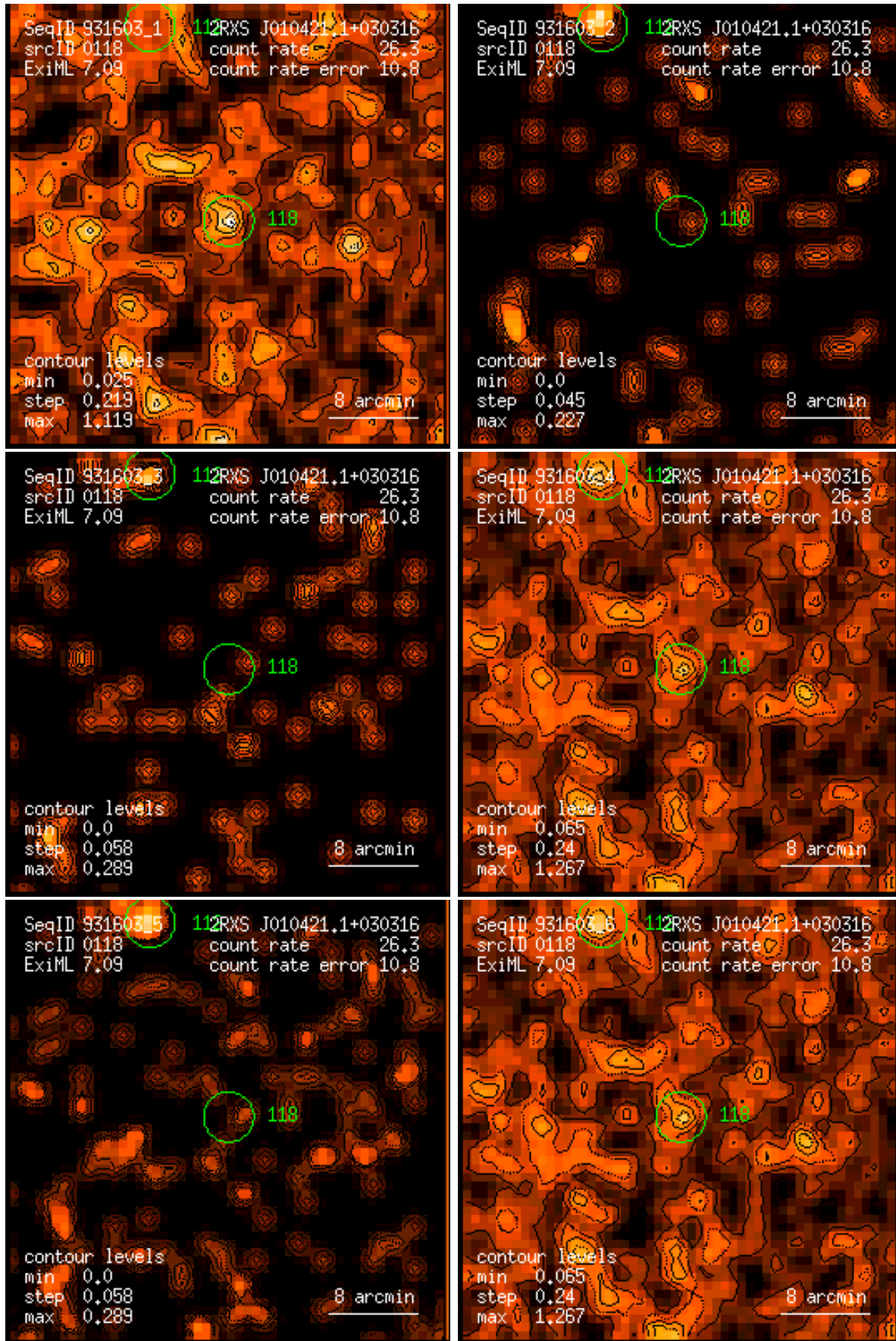
Figure 118: RASS 931603: detection 0118: band rate images, Gaussian filter: (1) PSPC channels 11 – 41, (2) 52 – 90, (3) 91 – 201, (4) 11 – 235, (5) 52 – 201, (6) 11 – 201. Broad band rates in counts/ks. Band rate contour levels in counts/ks/arcmin 2 .
